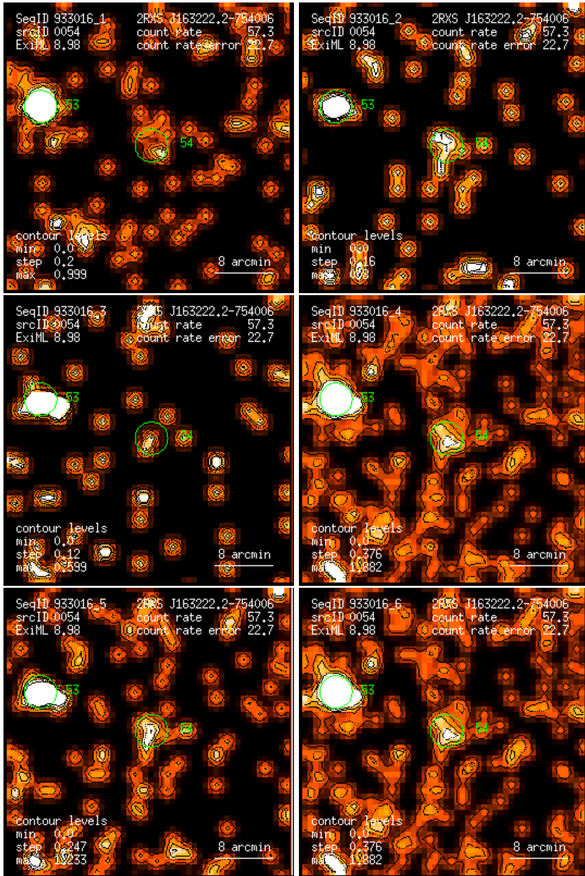
Figure 54: RASS 933016: detection 0054: band rate images, Gaussian filter: (1) PSPC channels 11 – 41, (2) 52 – 90, (3) 91 – 201, (4) 11 – 235, (5) 52 – 201, (6) 11 – 201. Broad band rates in counts/ks. Band rate contour levels in counts/ks/arcmin 2 .
