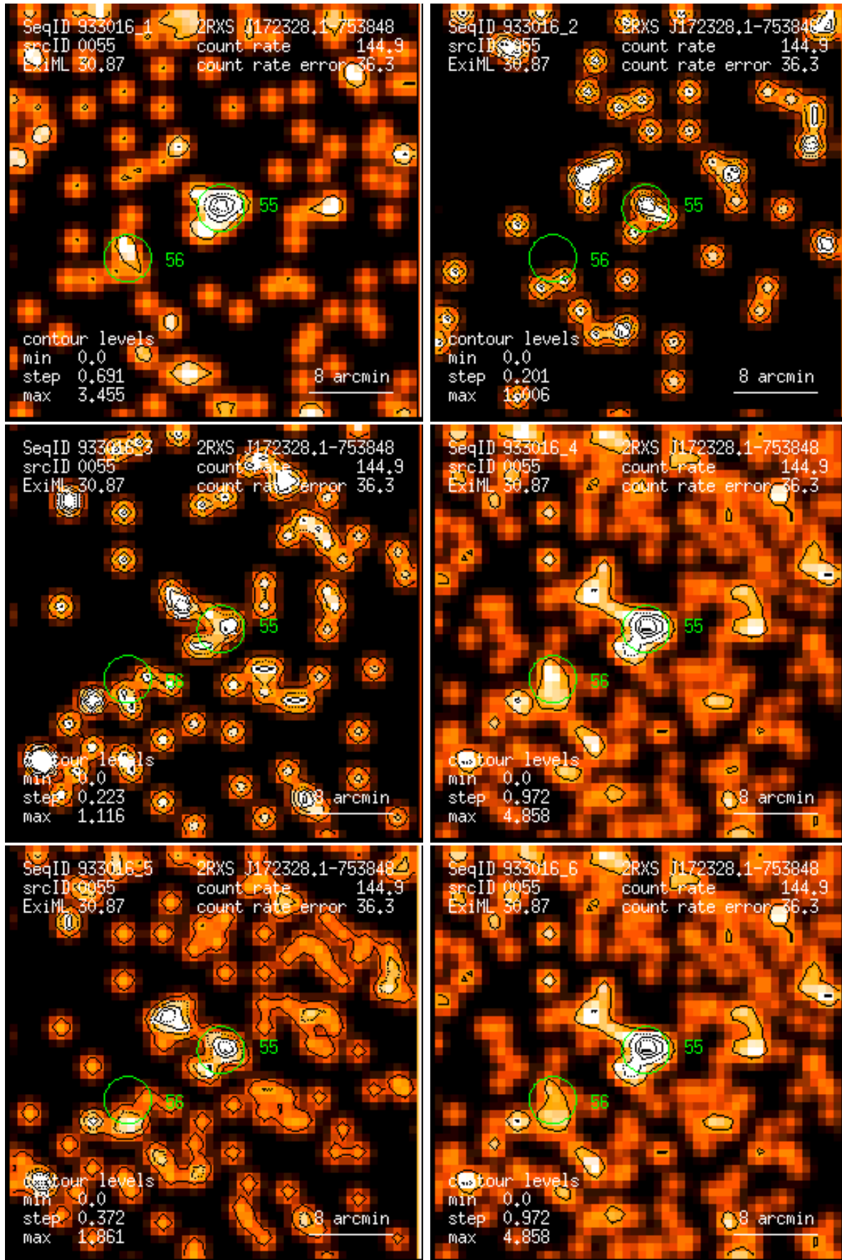
Figure 55: RASS 933016: detection 0055: band rate images, Gaussian filter: (1) PSPC channels 11 – 41, (2) 52 – 90, (3) 91 – 201, (4) 11 – 235, (5) 52 – 201, (6) 11 – 201. Broad band rates in counts/ks. Band rate contour levels in counts/ks/arcmin 2 .
