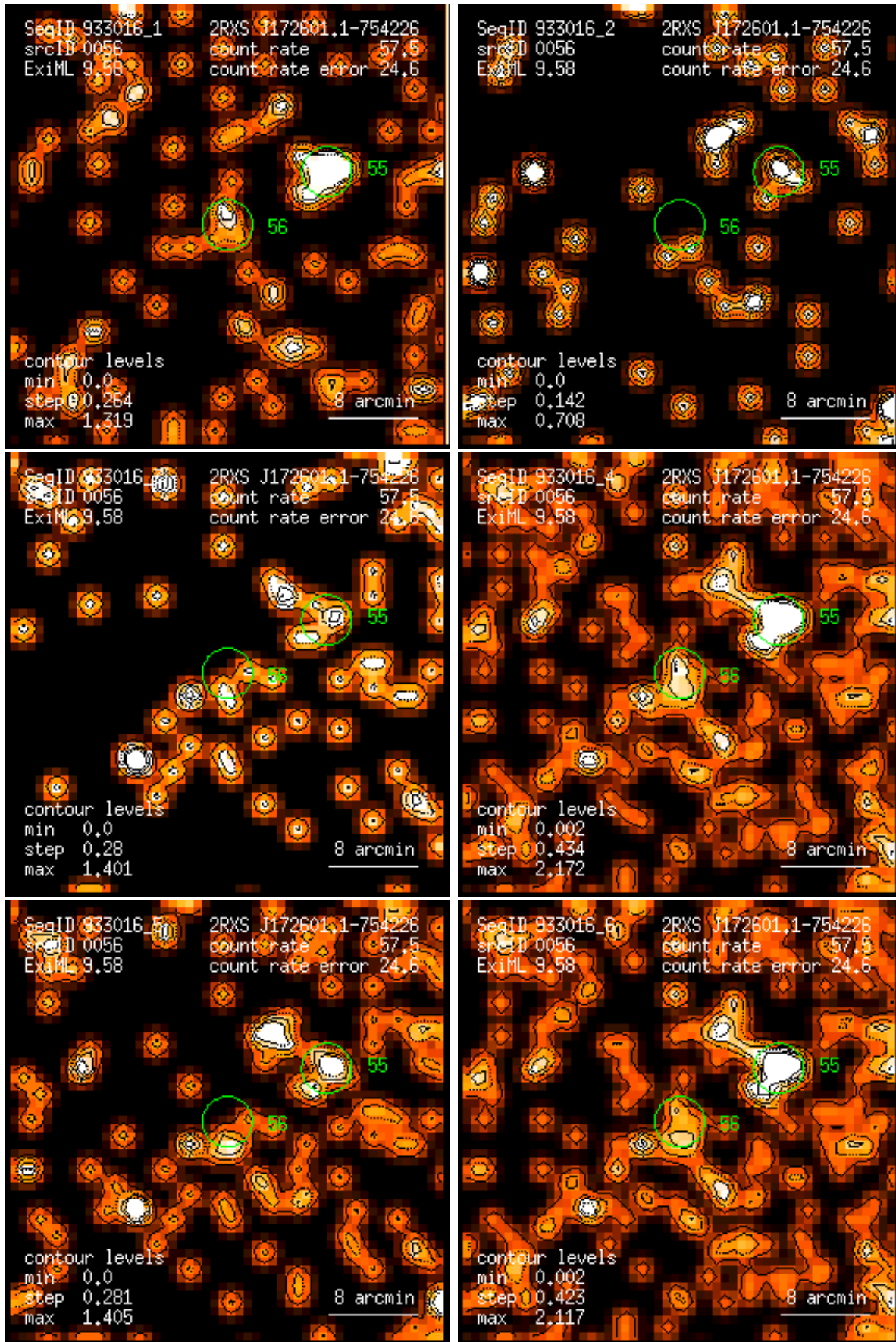
Figure 56: RASS 933016: detection 0056: band rate images, Gaussian filter: (1) PSPC channels 11 – 41, (2) 52 – 90, (3) 91 – 201, (4) 11 – 235, (5) 52 – 201, (6) 11 – 201. Broad band rates in counts/ks. Band rate contour levels in counts/ks/arcmin 2 .
