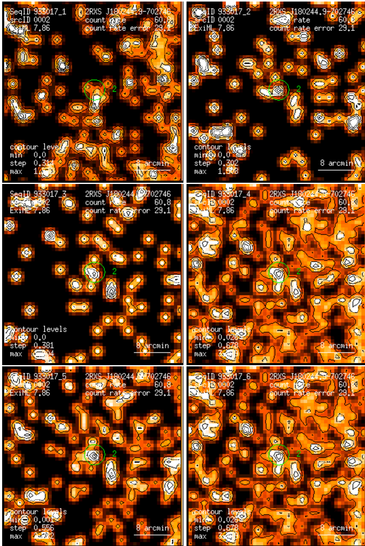
Figure 2: RASS 933017: detection 0002: band rate images, Gaussian filter: (1) PSPC channels 11 – 41, (2) 52 – 90, (3) 91 – 201, (4) 11 – 235, (5) 52 – 201, (6) 11 – 201. Broad band rates in counts/ks. Band rate contour levels in counts/ks/arcmin 2 .
