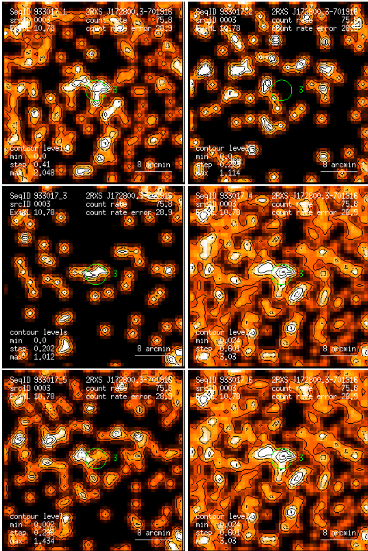
Figure 3: RASS 933017: detection 0003: band rate images, Gaussian filter: (1) PSPC channels 11 – 41, (2) 52 – 90, (3) 91 – 201, (4) 11 – 235, (5) 52 – 201, (6) 11 – 201. Broad band rates in counts/ks. Band rate contour levels in counts/ks/arcmin 2 .
