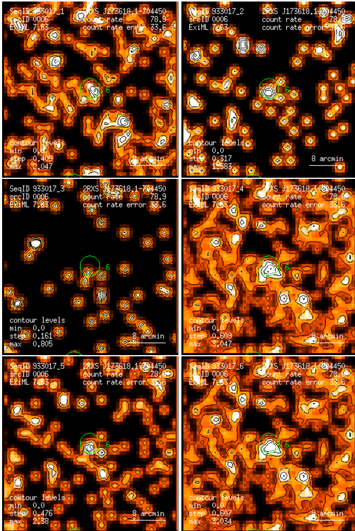
Figure 6: RASS 933017: detection 0006: band rate images, Gaussian filter: (1) PSPC channels 11 – 41, (2) 52 – 90, (3) 91 – 201, (4) 11 – 235, (5) 52 – 201, (6) 11 – 201. Broad band rates in counts/ks. Band rate contour levels in counts/ks/arcmin 2 .
