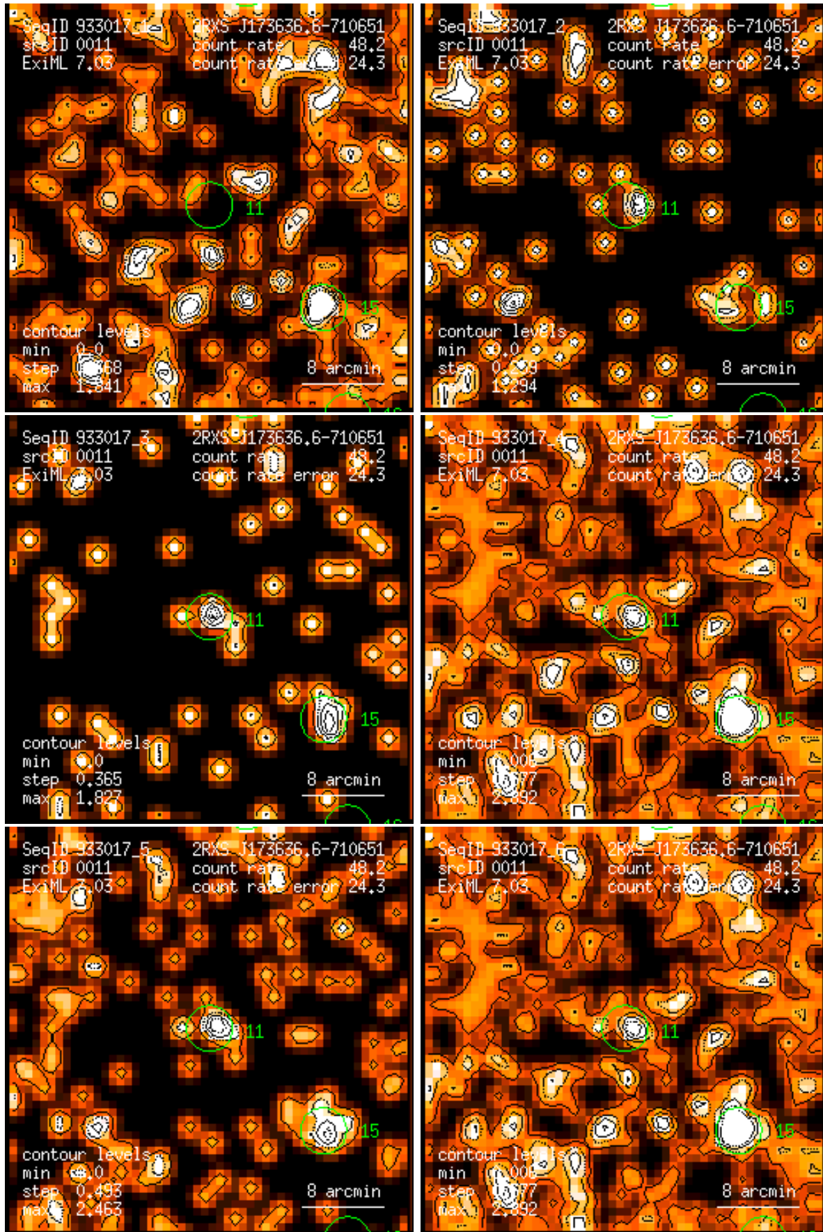
Figure 11: RASS 933017: detection 0011: band rate images, Gaussian filter: (1) PSPC channels 11 – 41, (2) 52 – 90, (3) 91 – 201, (4) 11 – 235, (5) 52 – 201, (6) 11 – 201. Broad band rates in counts/ks. Band rate contour levels in counts/ks/arcmin 2 .
