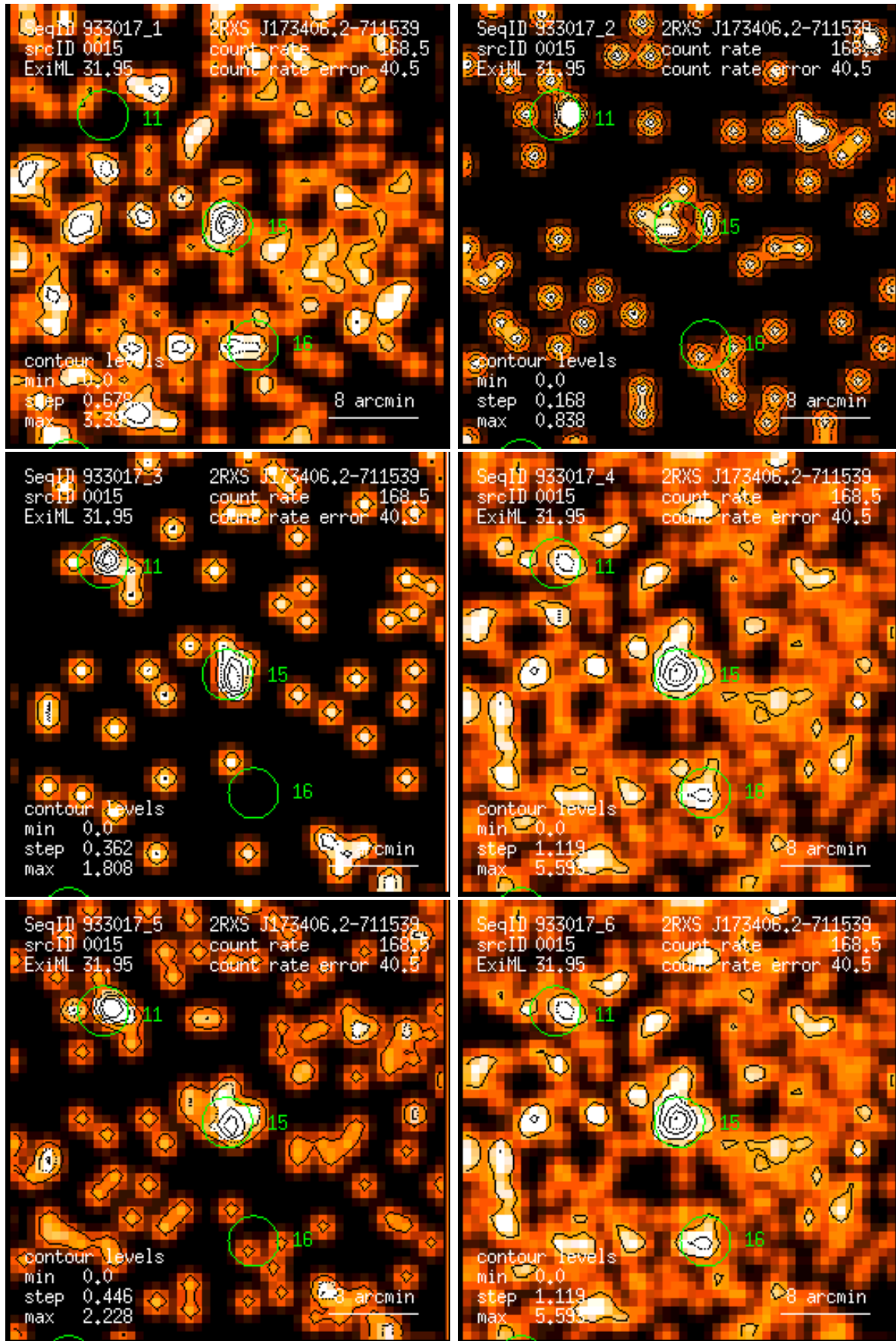
Figure 15: RASS 933017: detection 0015: band rate images, Gaussian filter: (1) PSPC channels 11 – 41, (2) 52 – 90, (3) 91 – 201, (4) 11 – 235, (5) 52 – 201, (6) 11 – 201. Broad band rates in counts/ks. Band rate contour levels in counts/ks/arcmin 2 .
