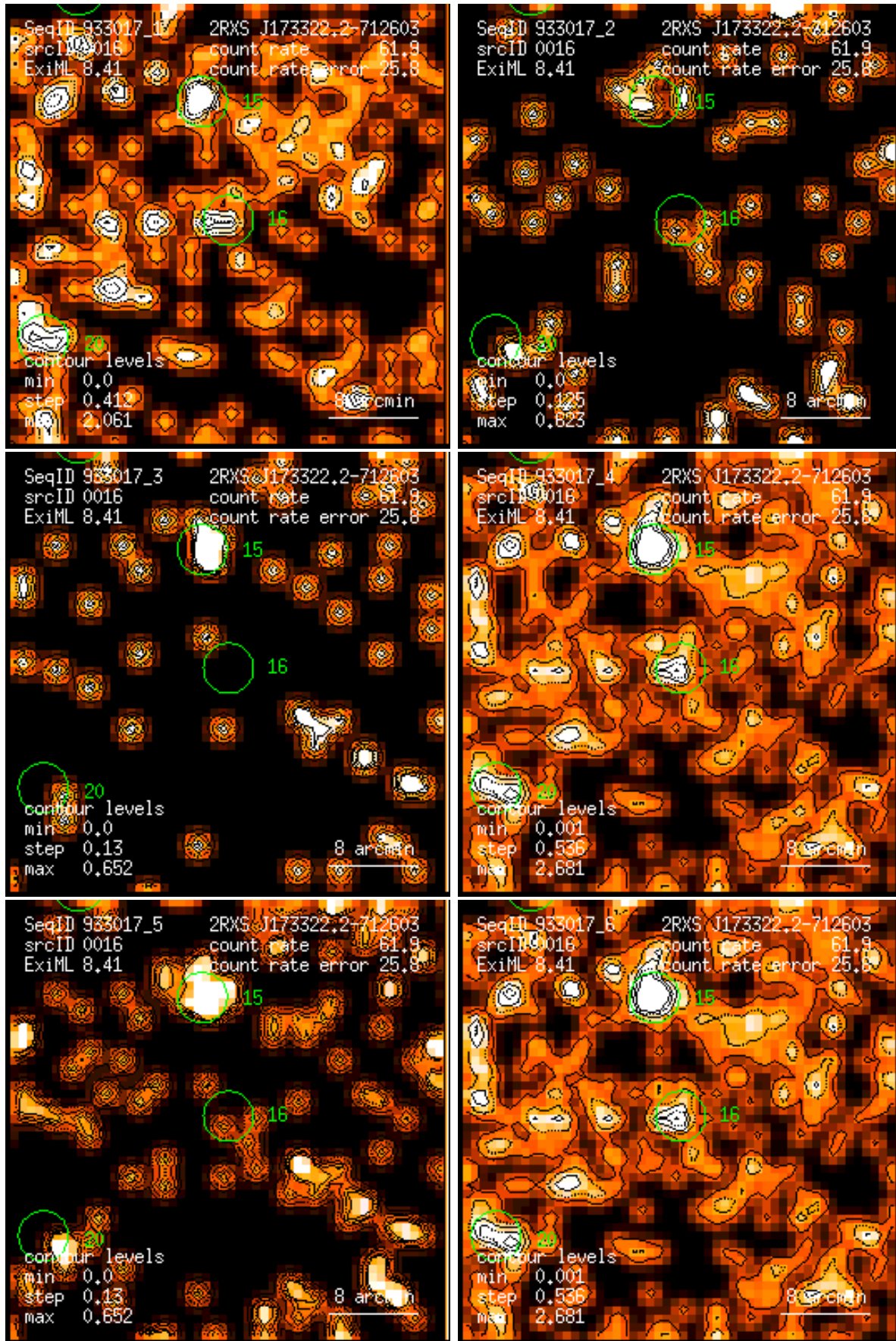
Figure 16: RASS 933017: detection 0016: band rate images, Gaussian filter: (1) PSPC channels 11 – 41, (2) 52 – 90, (3) 91 – 201, (4) 11 – 235, (5) 52 – 201, (6) 11 – 201. Broad band rates in counts/ks. Band rate contour levels in counts/ks/arcmin 2 .
