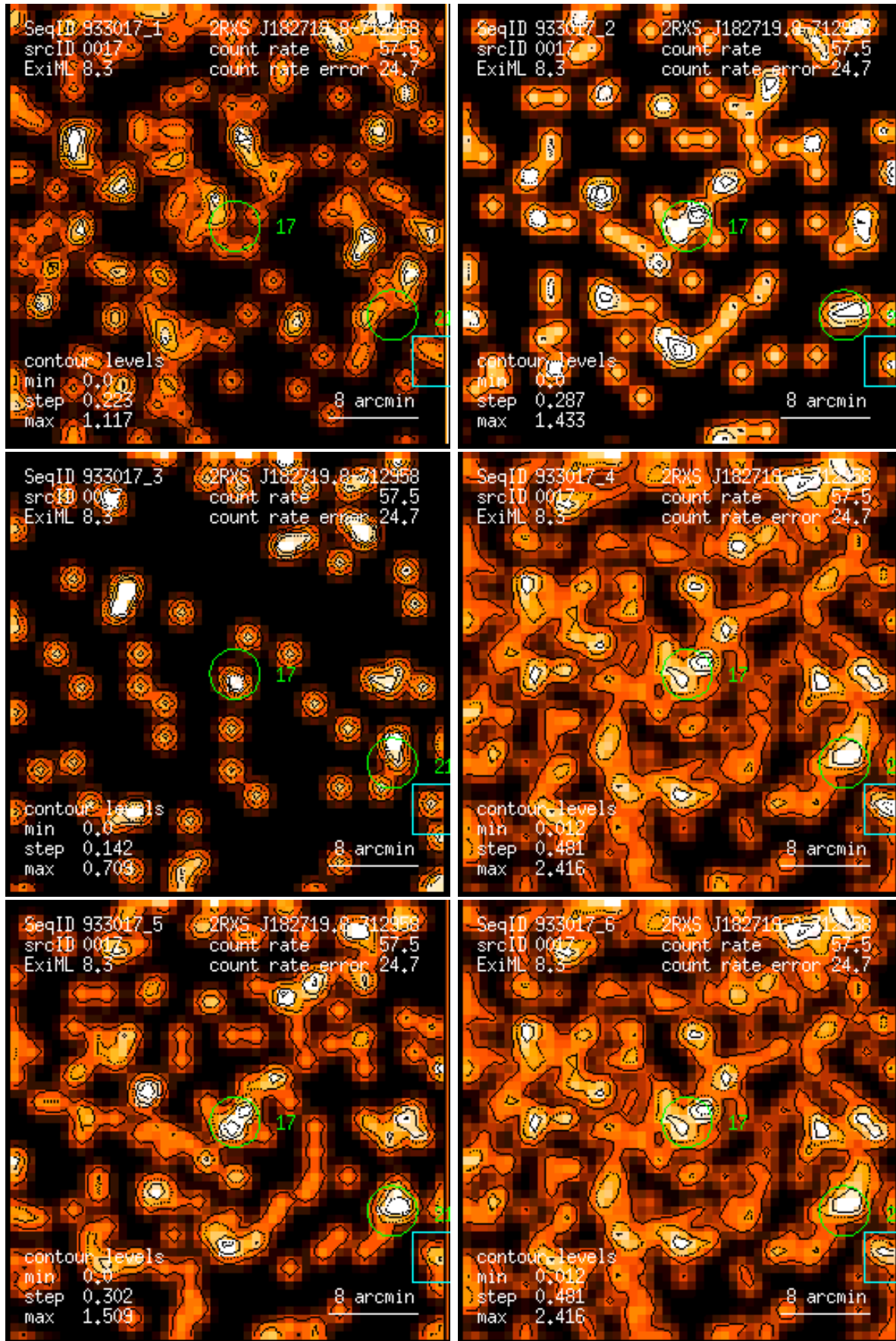
Figure 17: RASS 933017: detection 0017: band rate images, Gaussian filter: (1) PSPC channels 11 – 41, (2) 52 – 90, (3) 91 – 201, (4) 11 – 235, (5) 52 – 201, (6) 11 – 201. Broad band rates in counts/ks. Band rate contour levels in counts/ks/arcmin 2 .
