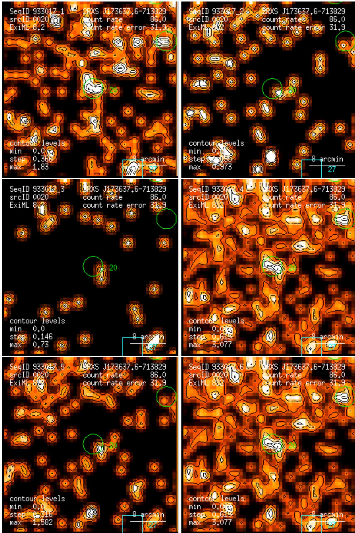
Figure 20: RASS 933017: detection 0020: band rate images, Gaussian filter: (1) PSPC channels 11 – 41, (2) 52 – 90, (3) 91 – 201, (4) 11 – 235, (5) 52 – 201, (6) 11 – 201. Broad band rates in counts/ks. Band rate contour levels in counts/ks/arcmin 2 .
