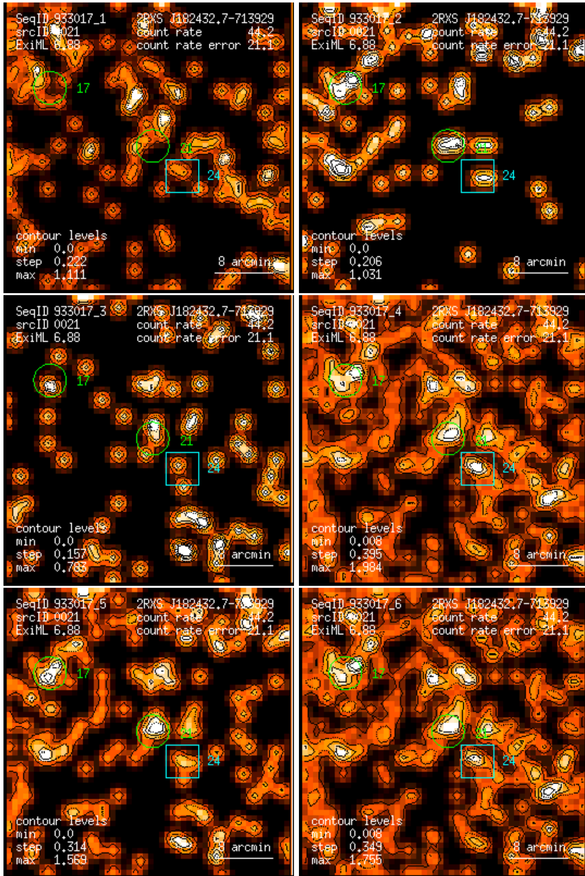
Figure 21: RASS 933017: detection 0021: band rate images, Gaussian filter: (1) PSPC channels 11 – 41, (2) 52 – 90, (3) 91 – 201, (4) 11 – 235, (5) 52 – 201, (6) 11 – 201. Broad band rates in counts/ks. Band rate contour levels in counts/ks/arcmin 2 .
