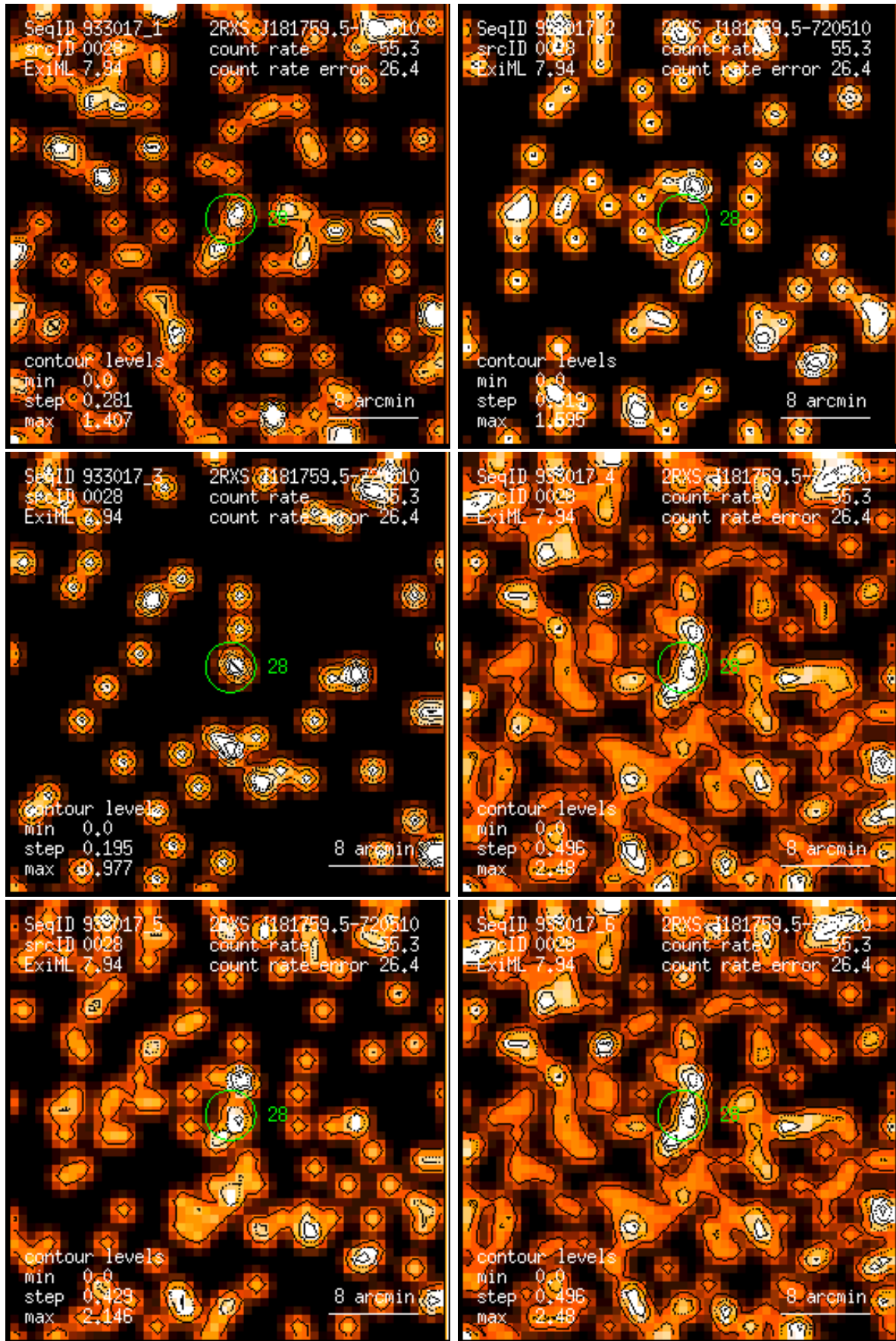
Figure 28: RASS 933017: detection 0028: band rate images, Gaussian filter: (1) PSPC channels 11 – 41, (2) 52 – 90, (3) 91 – 201, (4) 11 – 235, (5) 52 – 201, (6) 11 – 201. Broad band rates in counts/ks. Band rate contour levels in counts/ks/arcmin 2 .
