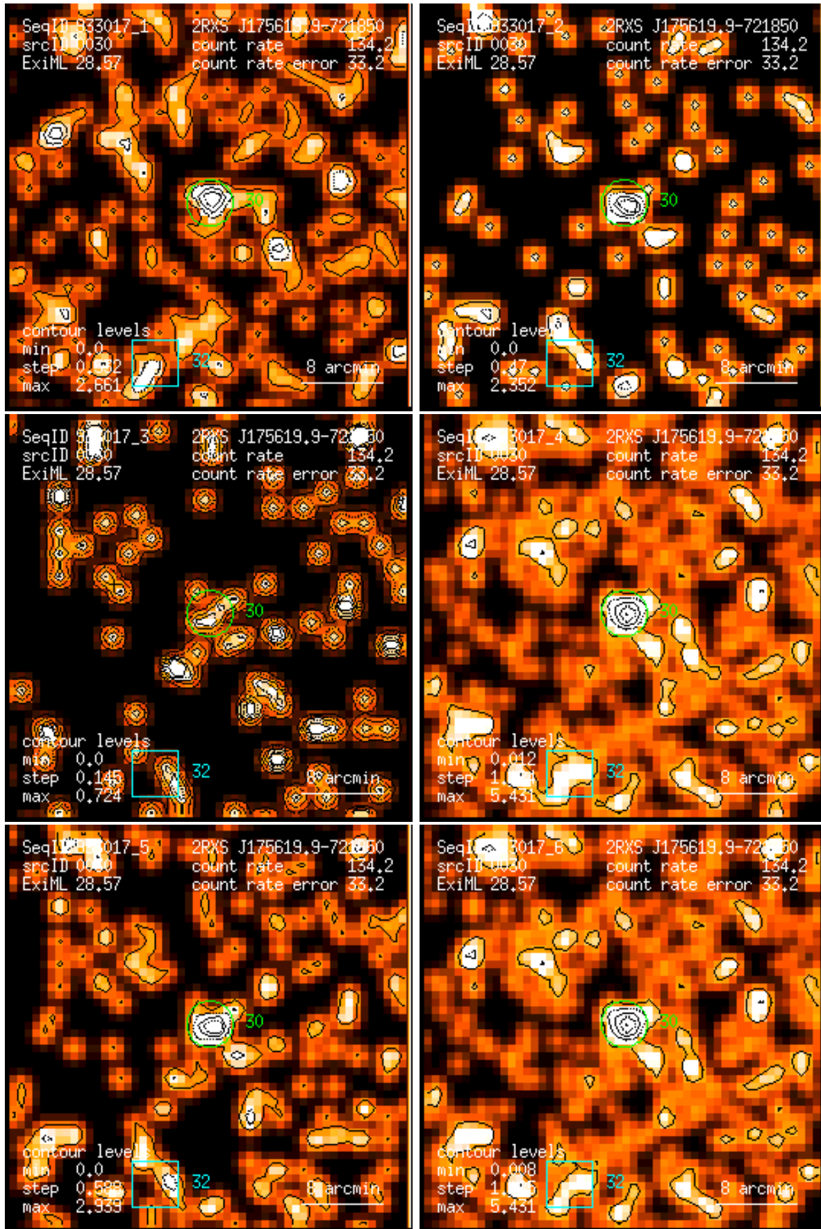
Figure 30: RASS 933017: detection 0030: band rate images, Gaussian filter: (1) PSPC channels 11 – 41, (2) 52 – 90, (3) 91 – 201, (4) 11 – 235, (5) 52 – 201, (6) 11 – 201. Broad band rates in counts/ks. Band rate contour levels in counts/ks/arcmin 2 .
