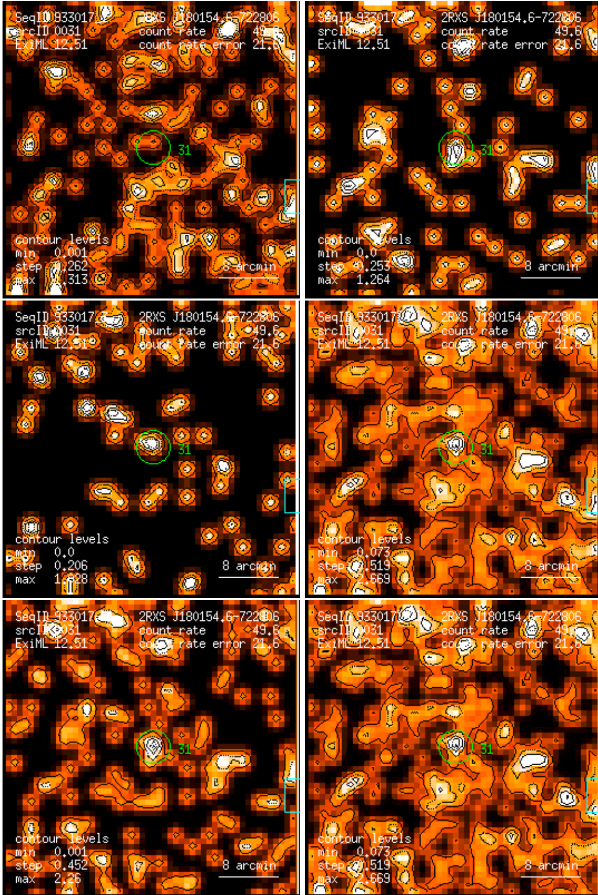
Figure 31: RASS 933017: detection 0031: band rate images, Gaussian filter: (1) PSPC channels 11 – 41, (2) 52 – 90, (3) 91 – 201, (4) 11 – 235, (5) 52 – 201, (6) 11 – 201. Broad band rates in counts/ks. Band rate contour levels in counts/ks/arcmin 2 .
