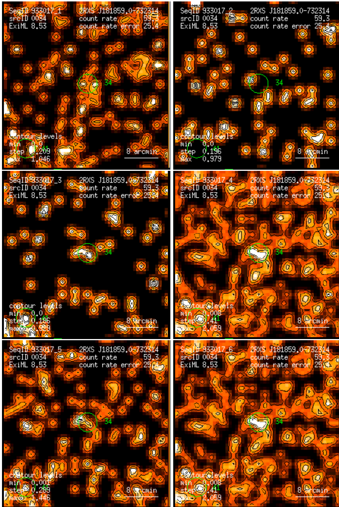
Figure 34: RASS 933017: detection 0034: band rate images, Gaussian filter: (1) PSPC channels 11 – 41, (2) 52 – 90, (3) 91 – 201, (4) 11 – 235, (5) 52 – 201, (6) 11 – 201. Broad band rates in counts/ks. Band rate contour levels in counts/ks/arcmin 2 .
