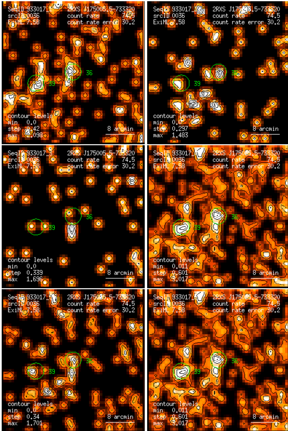
Figure 36: RASS 933017: detection 0036: band rate images, Gaussian filter: (1) PSPC channels 11 – 41, (2) 52 – 90, (3) 91 – 201, (4) 11 – 235, (5) 52 – 201, (6) 11 – 201. Broad band rates in counts/ks. Band rate contour levels in counts/ks/arcmin 2 .
