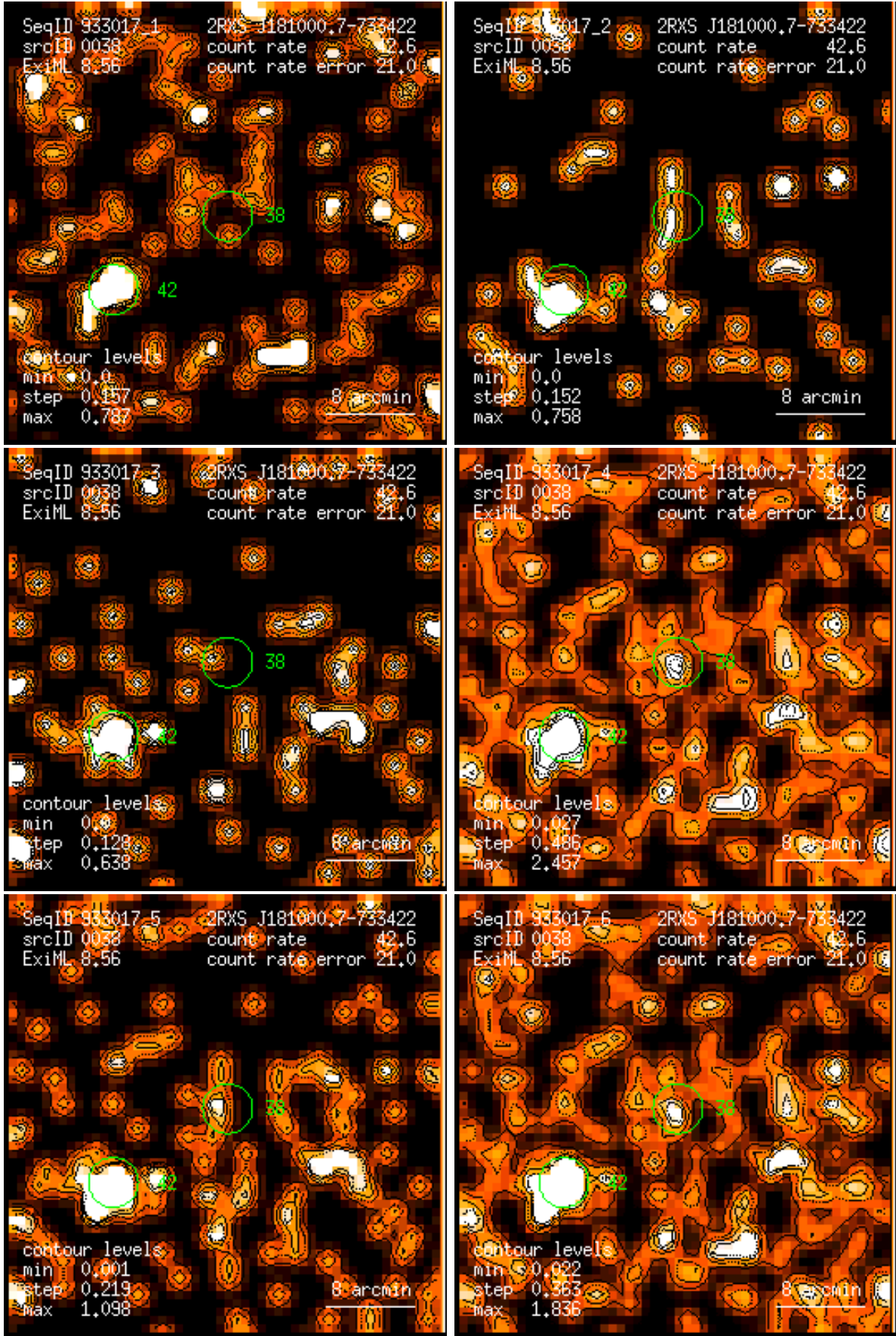
Figure 38: RASS 933017: detection 0038: band rate images, Gaussian filter: (1) PSPC channels 11 – 41, (2) 52 – 90, (3) 91 – 201, (4) 11 – 235, (5) 52 – 201, (6) 11 – 201. Broad band rates in counts/ks. Band rate contour levels in counts/ks/arcmin 2 .
