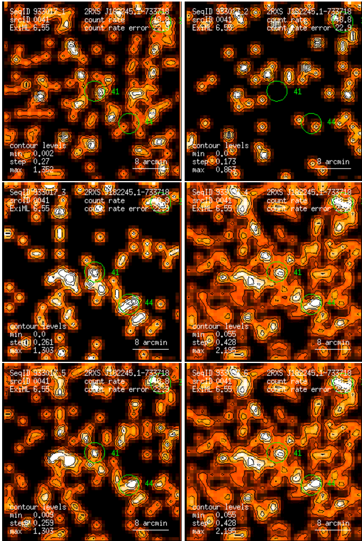
Figure 41: RASS 933017: detection 0041: band rate images, Gaussian filter: (1) PSPC channels 11 – 41, (2) 52 – 90, (3) 91 – 201, (4) 11 – 235, (5) 52 – 201, (6) 11 – 201. Broad band rates in counts/ks. Band rate contour levels in counts/ks/arcmin 2 .
