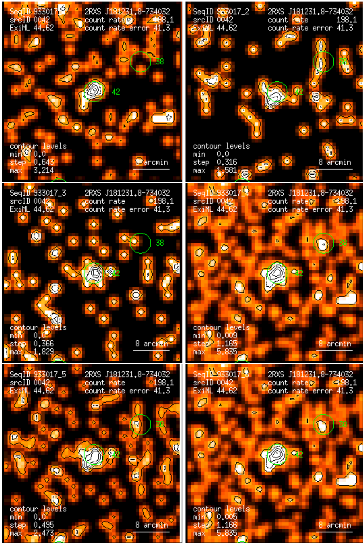
Figure 42: RASS 933017: detection 0042: band rate images, Gaussian filter: (1) PSPC channels 11 – 41, (2) 52 – 90, (3) 91 – 201, (4) 11 – 235, (5) 52 – 201, (6) 11 – 201. Broad band rates in counts/ks. Band rate contour levels in counts/ks/arcmin 2 .
