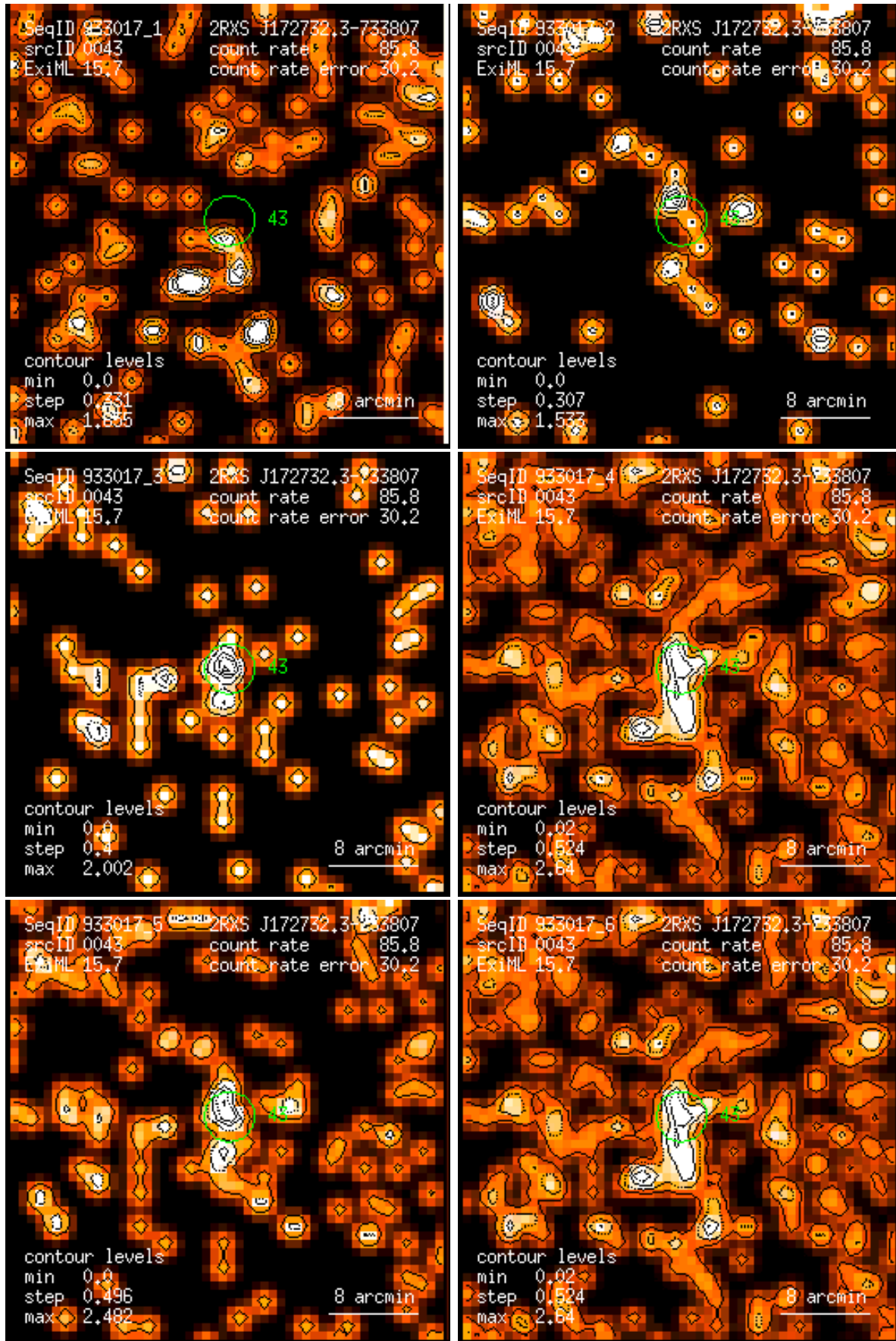
Figure 43: RASS 933017: detection 0043: band rate images, Gaussian filter: (1) PSPC channels 11 – 41, (2) 52 – 90, (3) 91 – 201, (4) 11 – 235, (5) 52 – 201, (6) 11 – 201. Broad band rates in counts/ks. Band rate contour levels in counts/ks/arcmin 2 .
