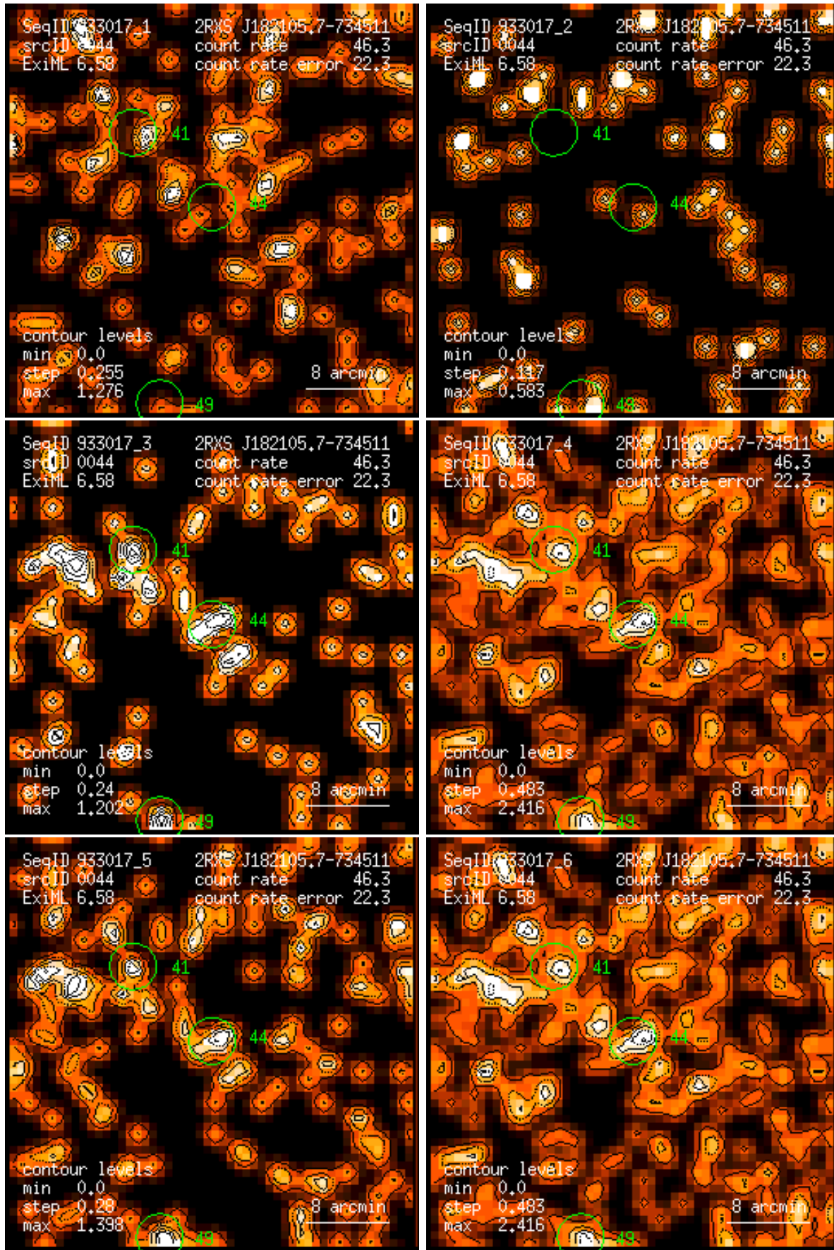
Figure 44: RASS 933017: detection 0044: band rate images, Gaussian filter: (1) PSPC channels 11 – 41, (2) 52 – 90, (3) 91 – 201, (4) 11 – 235, (5) 52 – 201, (6) 11 – 201. Broad band rates in counts/ks. Band rate contour levels in counts/ks/arcmin 2 .
