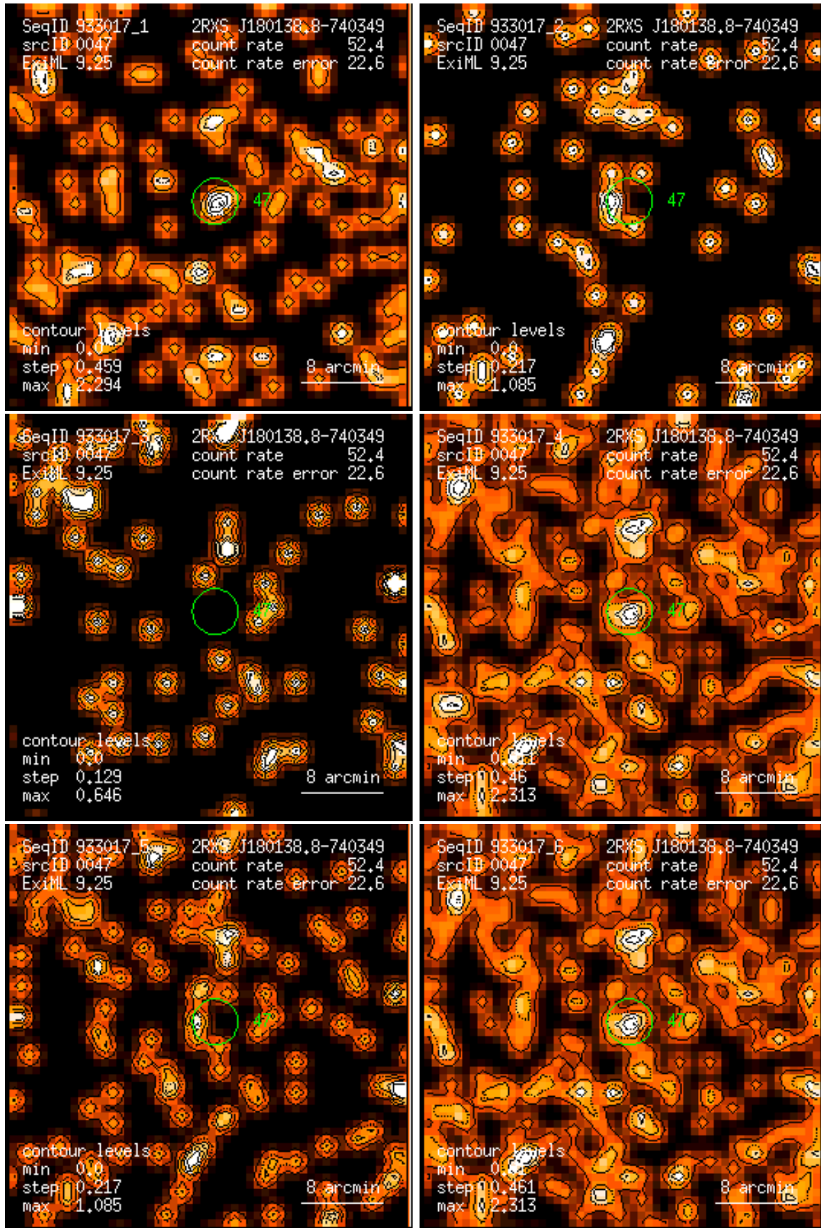
Figure 47: RASS 933017: detection 0047: band rate images, Gaussian filter: (1) PSPC channels 11 – 41, (2) 52 – 90, (3) 91 – 201, (4) 11 – 235, (5) 52 – 201, (6) 11 – 201. Broad band rates in counts/ks. Band rate contour levels in counts/ks/arcmin 2 .
