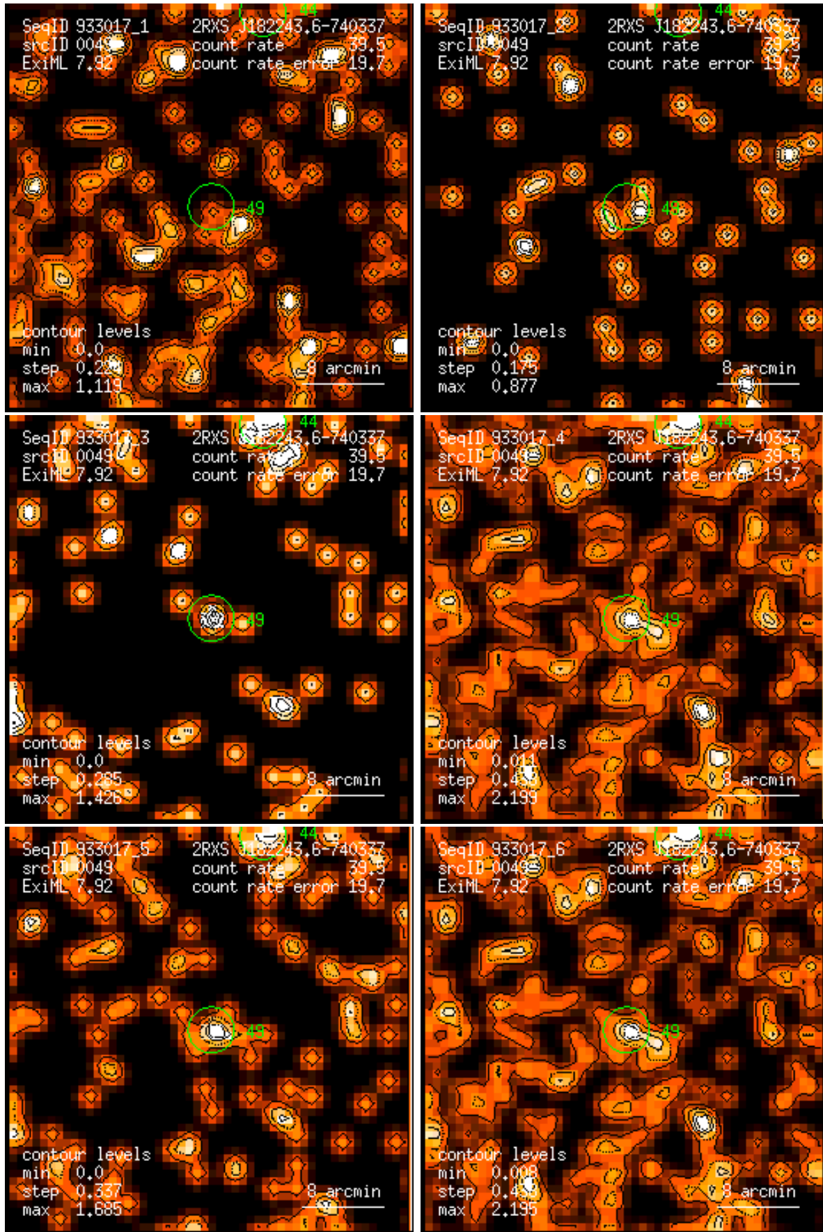
Figure 49: RASS 933017: detection 0049: band rate images, Gaussian filter: (1) PSPC channels 11 – 41, (2) 52 – 90, (3) 91 – 201, (4) 11 – 235, (5) 52 – 201, (6) 11 – 201. Broad band rates in counts/ks. Band rate contour levels in counts/ks/arcmin 2 .
