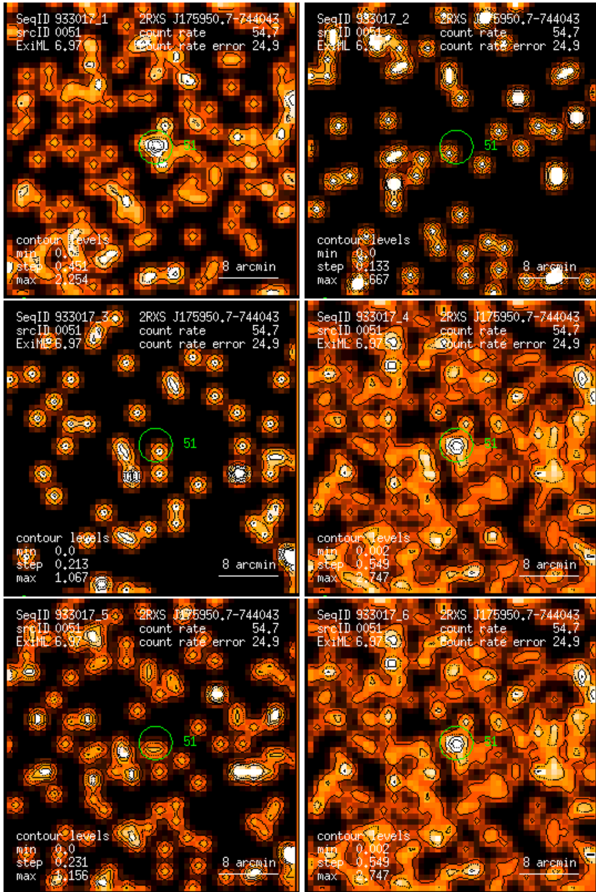
Figure 51: RASS 933017: detection 0051: band rate images, Gaussian filter: (1) PSPC channels 11 – 41, (2) 52 – 90, (3) 91 – 201, (4) 11 – 235, (5) 52 – 201, (6) 11 – 201. Broad band rates in counts/ks. Band rate contour levels in counts/ks/arcmin 2 .
