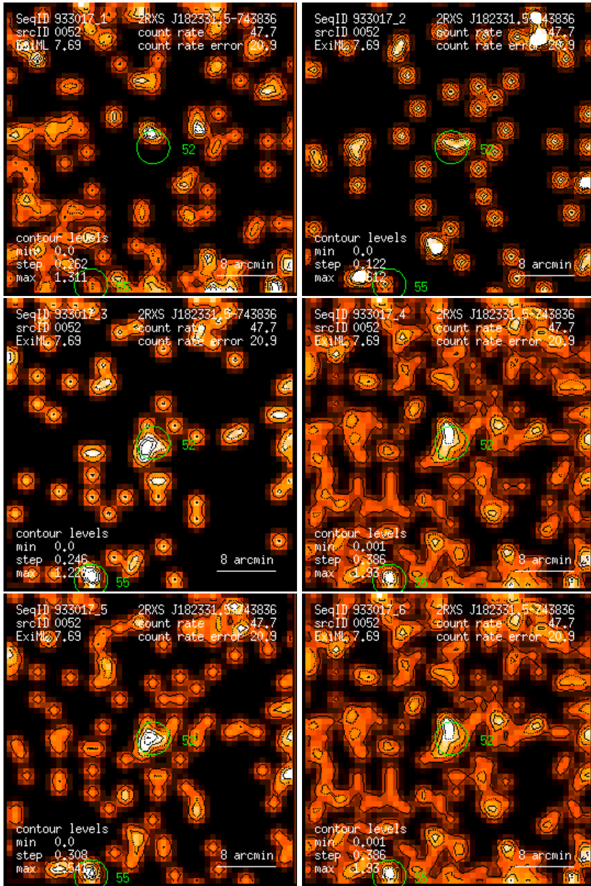
Figure 52: RASS 933017: detection 0052: band rate images, Gaussian filter: (1) PSPC channels 11 – 41, (2) 52 – 90, (3) 91 – 201, (4) 11 – 235, (5) 52 – 201, (6) 11 – 201. Broad band rates in counts/ks. Band rate contour levels in counts/ks/arcmin 2 .
