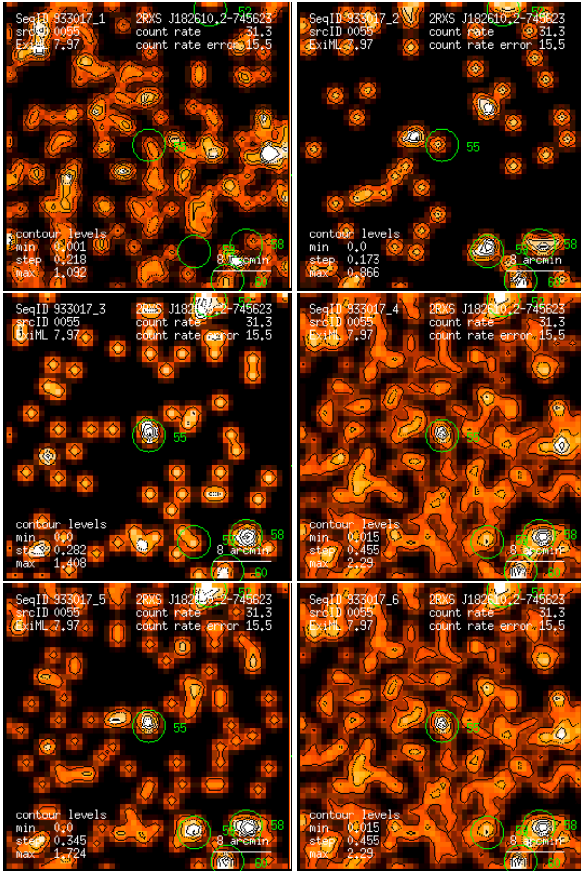
Figure 55: RASS 933017: detection 0055: band rate images, Gaussian filter: (1) PSPC channels 11 – 41, (2) 52 – 90, (3) 91 – 201, (4) 11 – 235, (5) 52 – 201, (6) 11 – 201. Broad band rates in counts/ks. Band rate contour levels in counts/ks/arcmin 2 .
