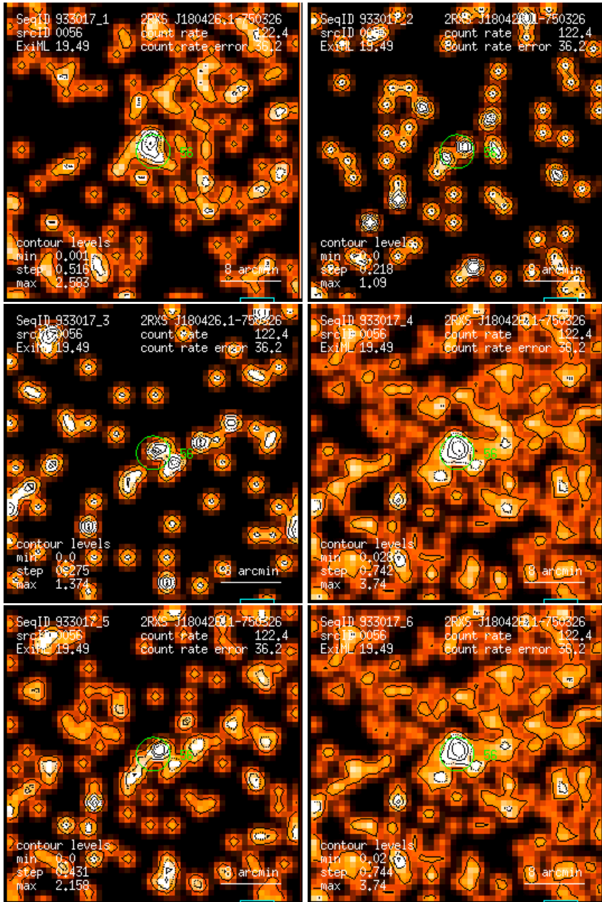
Figure 56: RASS 933017: detection 0056: band rate images, Gaussian filter: (1) PSPC channels 11 – 41, (2) 52 – 90, (3) 91 – 201, (4) 11 – 235, (5) 52 – 201, (6) 11 – 201. Broad band rates in counts/ks. Band rate contour levels in counts/ks/arcmin 2 .
