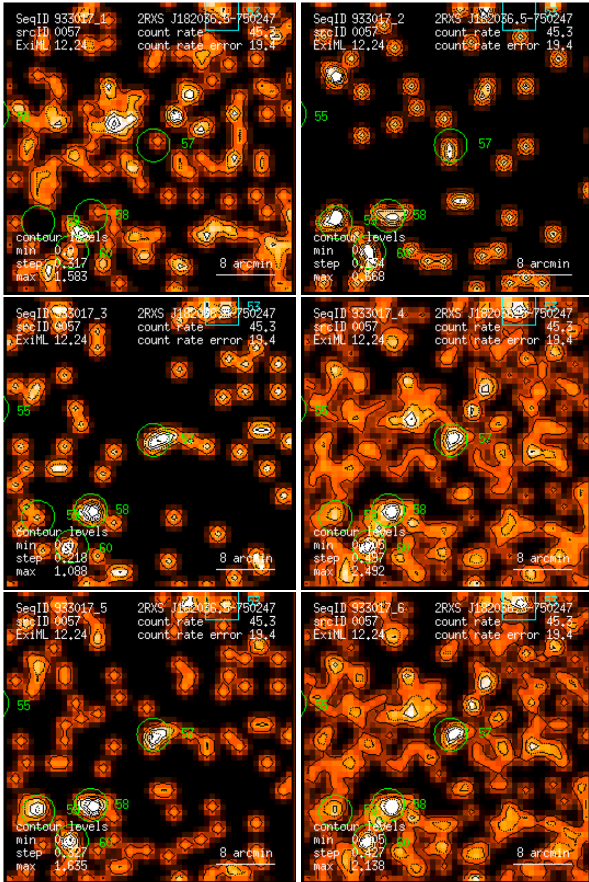
Figure 57: RASS 933017: detection 0057: band rate images, Gaussian filter: (1) PSPC channels 11 – 41, (2) 52 – 90, (3) 91 – 201, (4) 11 – 235, (5) 52 – 201, (6) 11 – 201. Broad band rates in counts/ks. Band rate contour levels in counts/ks/arcmin 2 .
