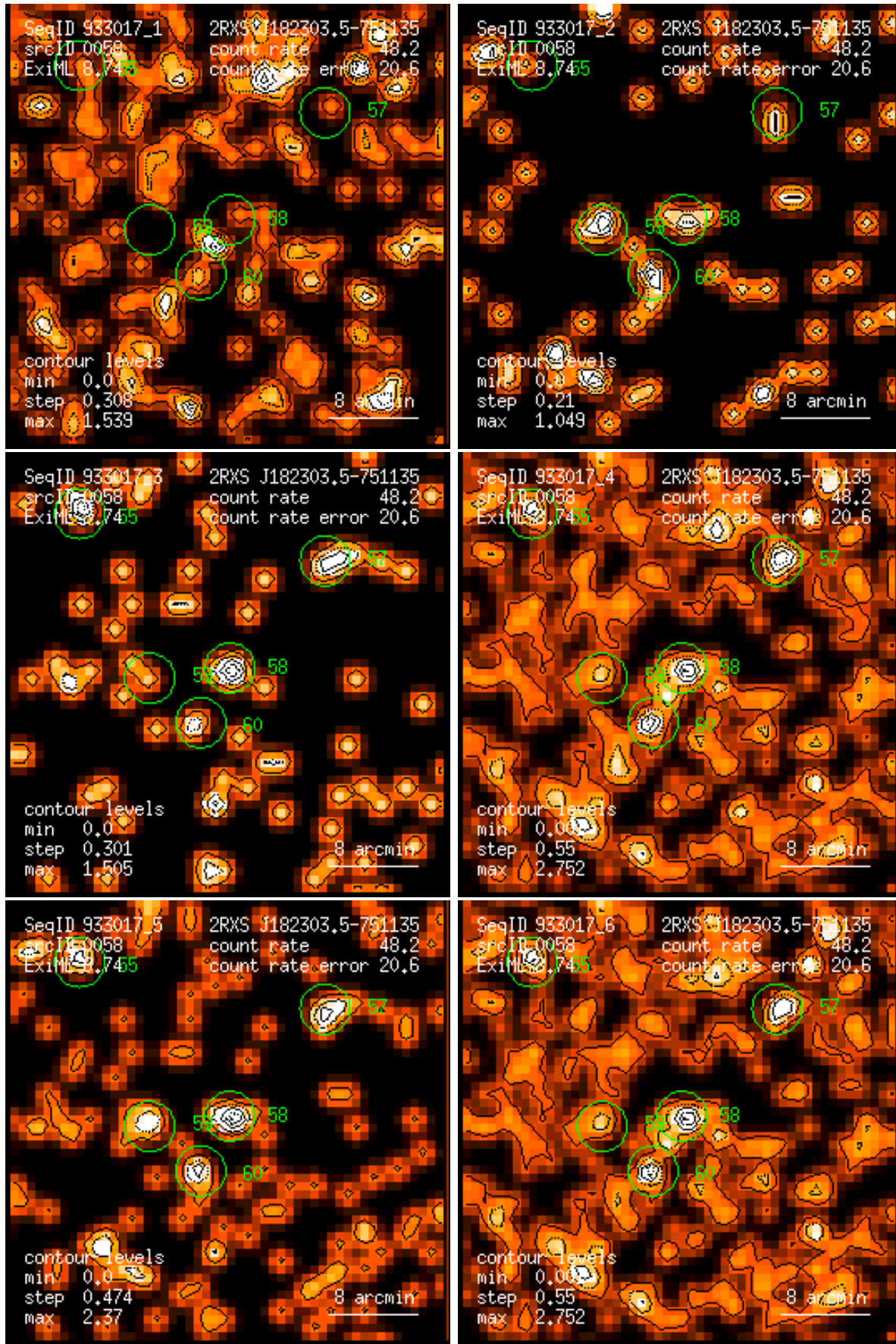
Figure 58: RASS 933017: detection 0058: band rate images, Gaussian filter: (1) PSPC channels 11 – 41, (2) 52 – 90, (3) 91 – 201, (4) 11 – 235, (5) 52 – 201, (6) 11 – 201. Broad band rates in counts/ks. Band rate contour levels in counts/ks/arcmin 2 .
