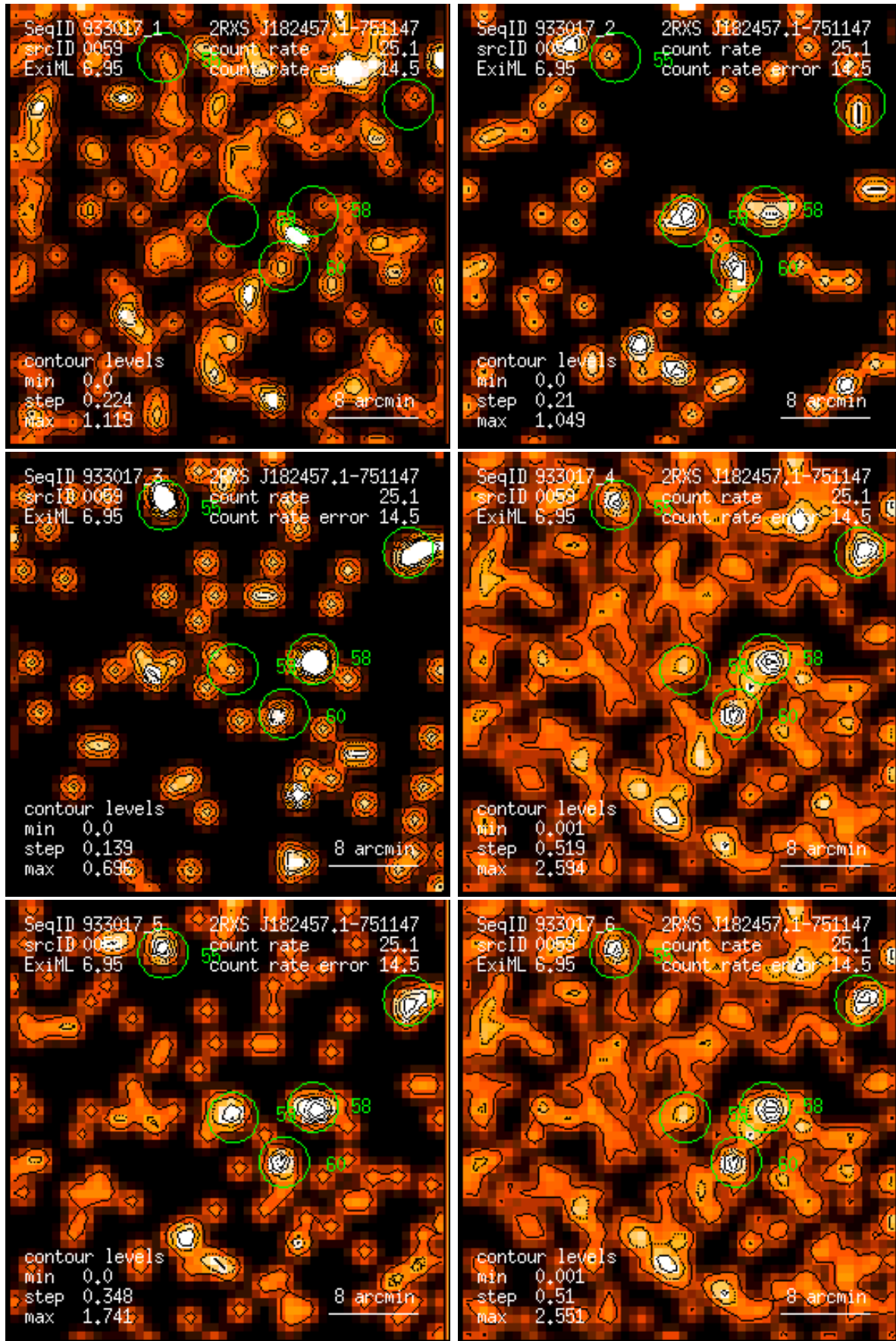
Figure 59: RASS 933017: detection 0059: band rate images, Gaussian filter: (1) PSPC channels 11 – 41, (2) 52 – 90, (3) 91 – 201, (4) 11 – 235, (5) 52 – 201, (6) 11 – 201. Broad band rates in counts/ks. Band rate contour levels in counts/ks/arcmin 2 .
