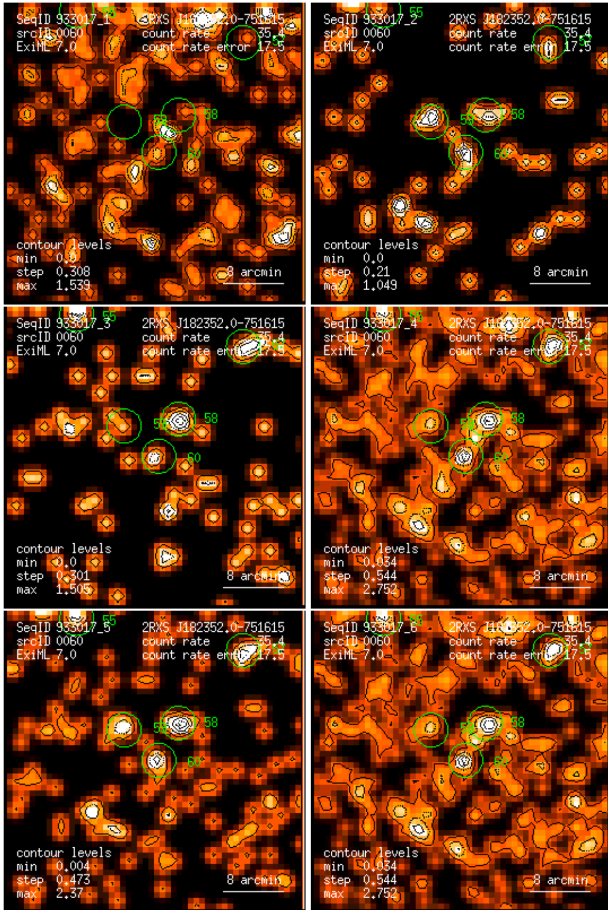
Figure 60: RASS 933017: detection 0060: band rate images, Gaussian filter: (1) PSPC channels 11 – 41, (2) 52 – 90, (3) 91 – 201, (4) 11 – 235, (5) 52 – 201, (6) 11 – 201. Broad band rates in counts/ks. Band rate contour levels in counts/ks/arcmin 2 .
