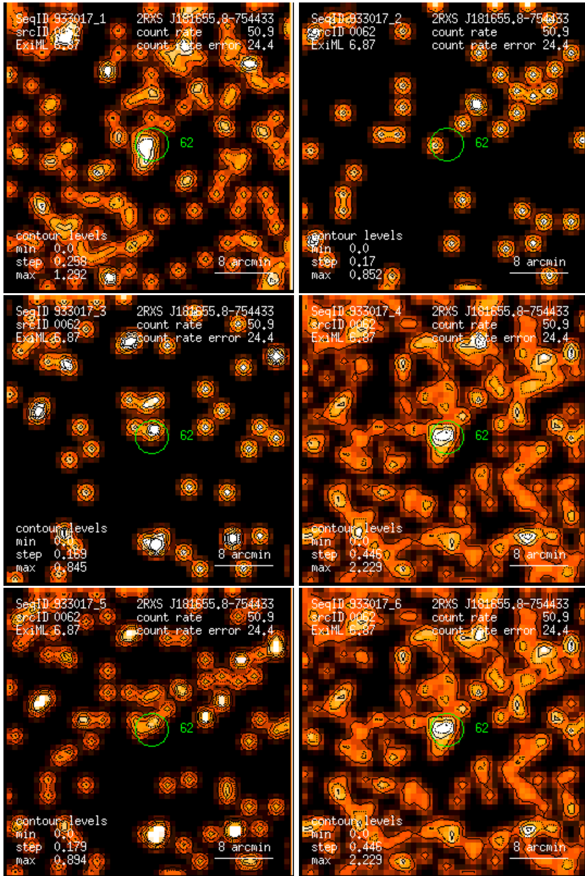
Figure 62: RASS 933017: detection 0062: band rate images, Gaussian filter: (1) PSPC channels 11 – 41, (2) 52 – 90, (3) 91 – 201, (4) 11 – 235, (5) 52 – 201, (6) 11 – 201. Broad band rates in counts/ks. Band rate contour levels in counts/ks/arcmin 2 .
