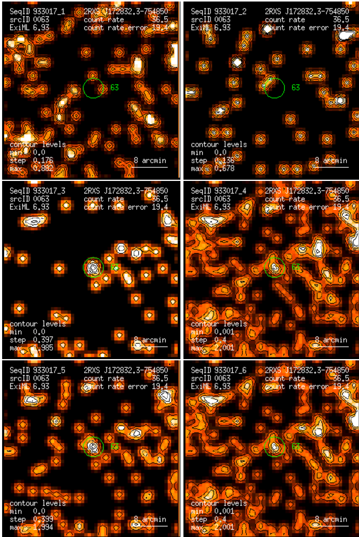
Figure 63: RASS 933017: detection 0063: band rate images, Gaussian filter: (1) PSPC channels 11 – 41, (2) 52 – 90, (3) 91 – 201, (4) 11 – 235, (5) 52 – 201, (6) 11 – 201. Broad band rates in counts/ks. Band rate contour levels in counts/ks/arcmin 2 .
