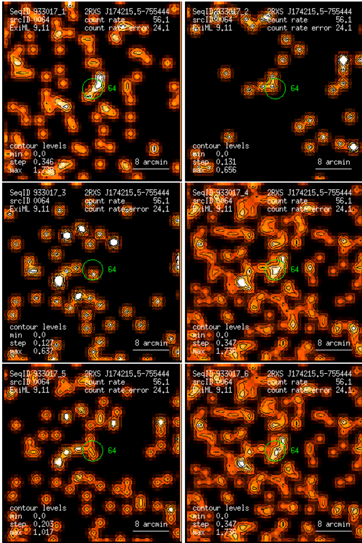
Figure 64: RASS 933017: detection 0064: band rate images, Gaussian filter: (1) PSPC channels 11 – 41, (2) 52 – 90, (3) 91 – 201, (4) 11 – 235, (5) 52 – 201, (6) 11 – 201. Broad band rates in counts/ks. Band rate contour levels in counts/ks/arcmin 2 .
