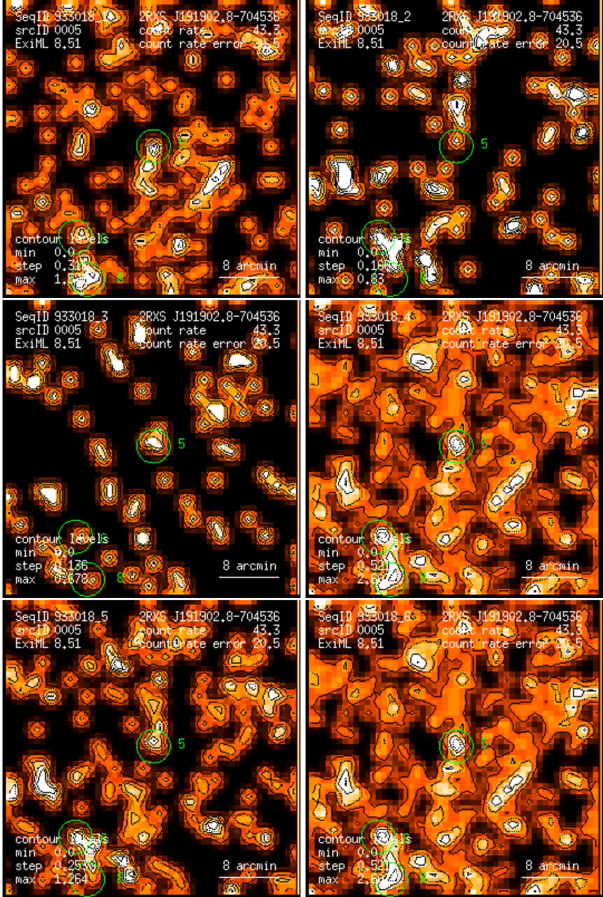
Figure 5: RASS 933018: detection 0005: band rate images, Gaussian filter: (1) PSPC channels 11 – 41, (2) 52 – 90, (3) 91 – 201, (4) 11 – 235, (5) 52 – 201, (6) 11 – 201. Broad band rates in counts/ks. Band rate contour levels in counts/ks/arcmin 2 .
