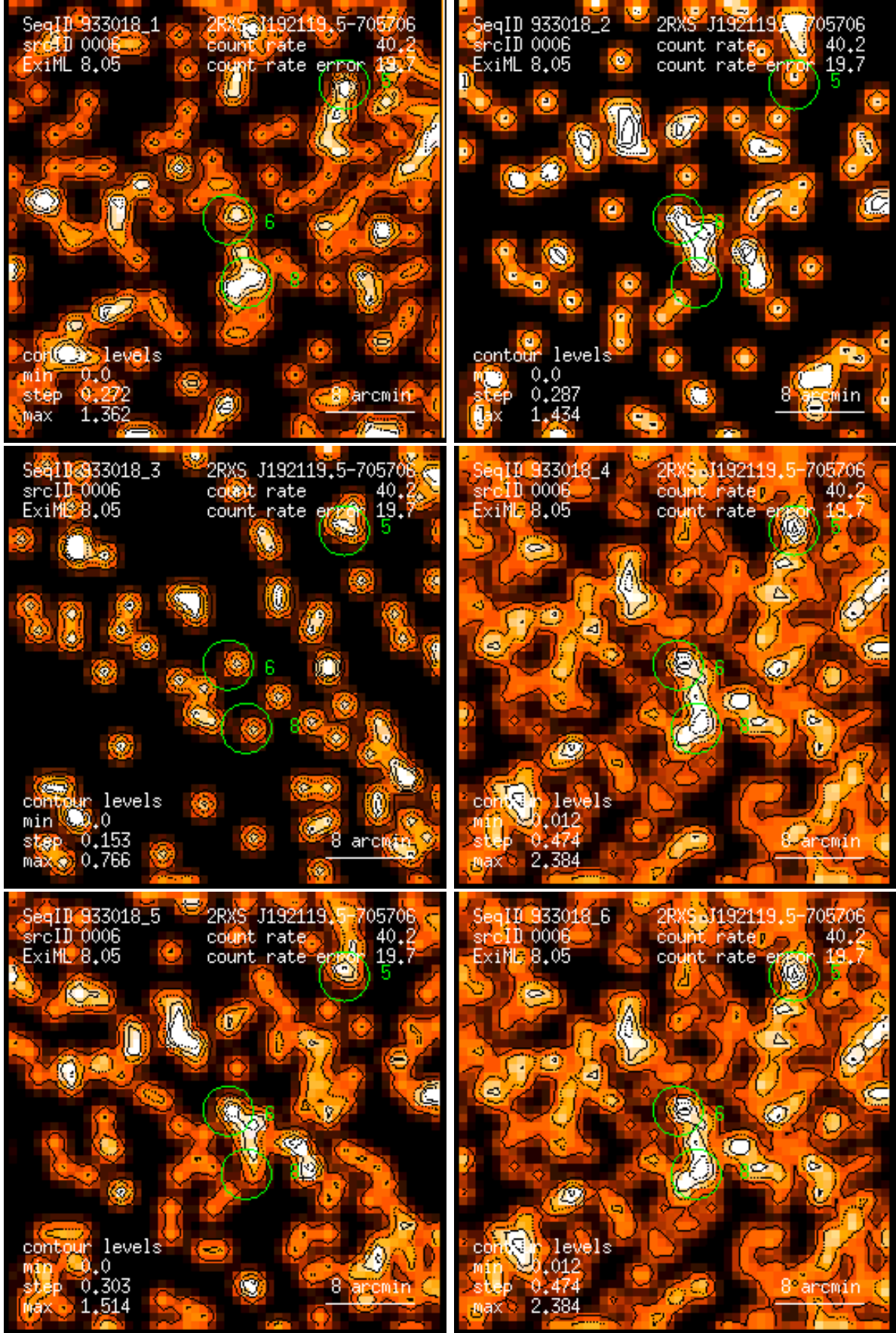
Figure 6: RASS 933018: detection 0006: band rate images, Gaussian filter: (1) PSPC channels 11 – 41, (2) 52 – 90, (3) 91 – 201, (4) 11 – 235, (5) 52 – 201, (6) 11 – 201. Broad band rates in counts/ks. Band rate contour levels in counts/ks/arcmin 2 .
