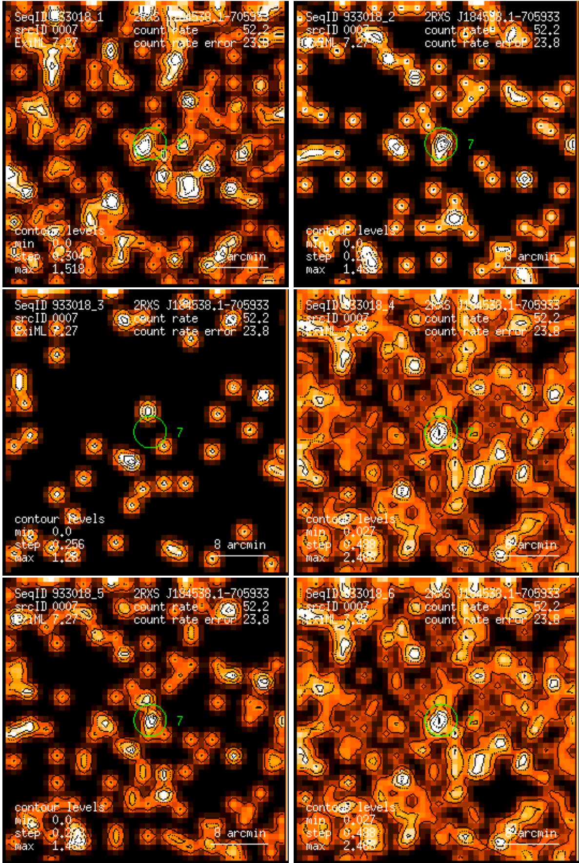
Figure 7: RASS 933018: detection 0007: band rate images, Gaussian filter: (1) PSPC channels 11 – 41, (2) 52 – 90, (3) 91 – 201, (4) 11 – 235, (5) 52 – 201, (6) 11 – 201. Broad band rates in counts/ks. Band rate contour levels in counts/ks/arcmin 2 .
