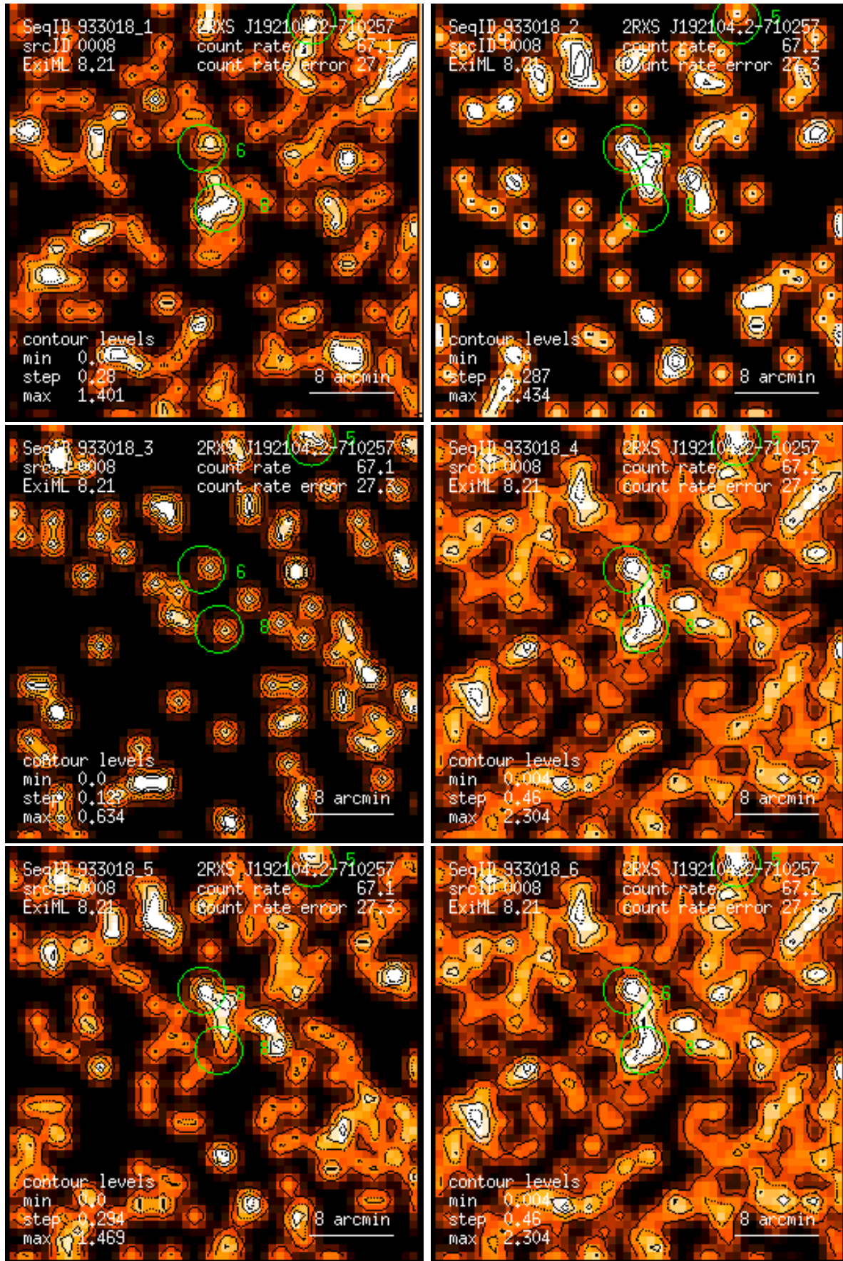
Figure 8: RASS 933018: detection 0008: band rate images, Gaussian filter: (1) PSPC channels 11 – 41, (2) 52 – 90, (3) 91 – 201, (4) 11 – 235, (5) 52 – 201, (6) 11 – 201. Broad band rates in counts/ks. Band rate contour levels in counts/ks/arcmin 2 .
