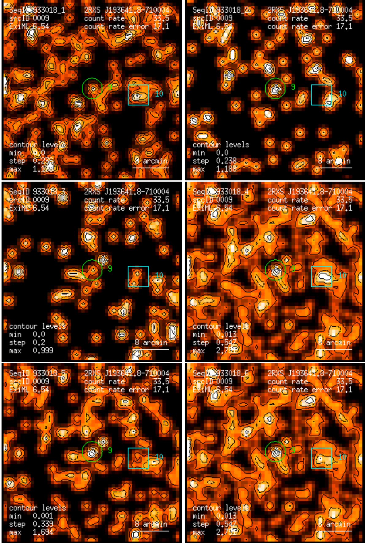
Figure 9: RASS 933018: detection 0009: band rate images, Gaussian filter: (1) PSPC channels 11 – 41, (2) 52 – 90, (3) 91 – 201, (4) 11 – 235, (5) 52 – 201, (6) 11 – 201. Broad band rates in counts/ks. Band rate contour levels in counts/ks/arcmin 2 .
