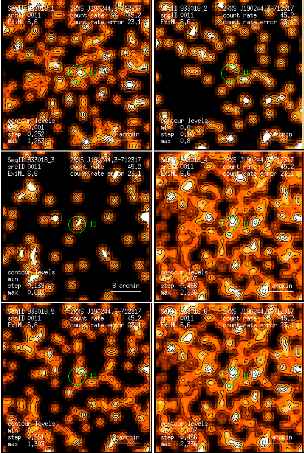
Figure 11: RASS 933018: detection 0011: band rate images, Gaussian filter: (1) PSPC channels 11 – 41, (2) 52 – 90, (3) 91 – 201, (4) 11 – 235, (5) 52 – 201, (6) 11 – 201. Broad band rates in counts/ks. Band rate contour levels in counts/ks/arcmin 2 .
