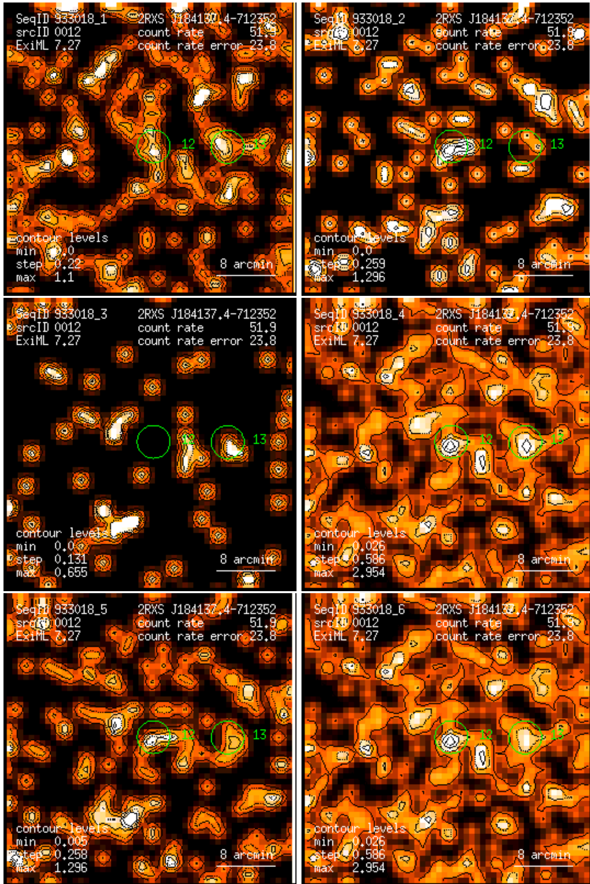
Figure 12: RASS 933018: detection 0012: band rate images, Gaussian filter: (1) PSPC channels 11 – 41, (2) 52 – 90, (3) 91 – 201, (4) 11 – 235, (5) 52 – 201, (6) 11 – 201. Broad band rates in counts/ks. Band rate contour levels in counts/ks/arcmin 2 .
