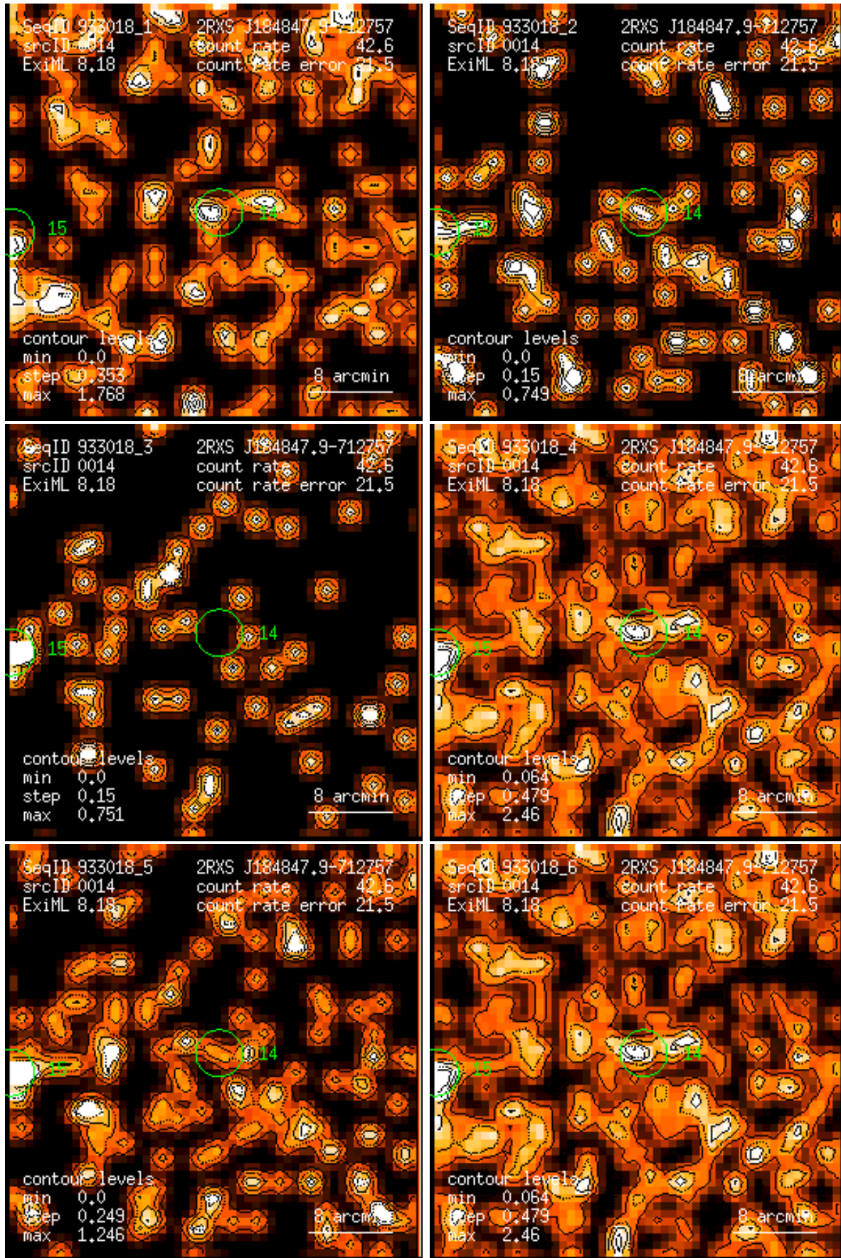
Figure 14: RASS 933018: detection 0014: band rate images, Gaussian filter: (1) PSPC channels 11 – 41, (2) 52 – 90, (3) 91 – 201, (4) 11 – 235, (5) 52 – 201, (6) 11 – 201. Broad band rates in counts/ks. Band rate contour levels in counts/ks/arcmin 2 .
