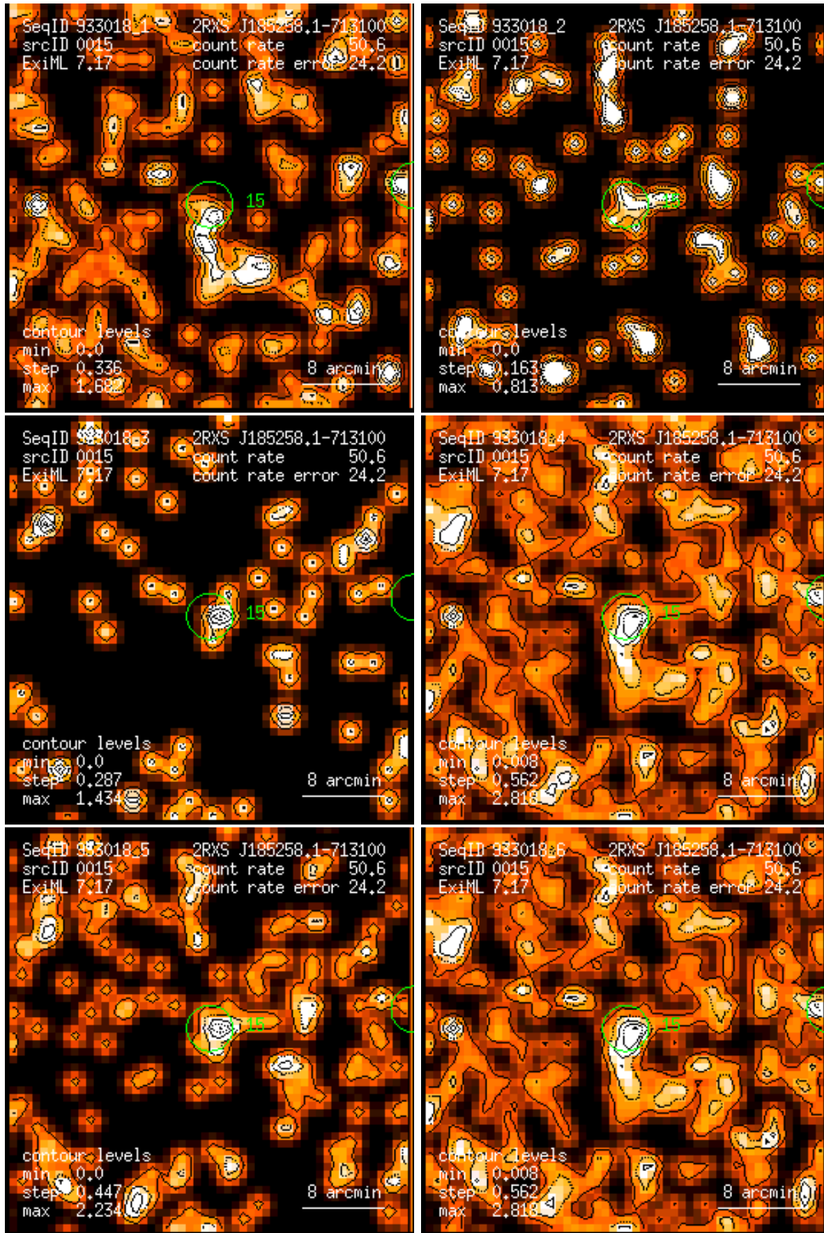
Figure 15: RASS 933018: detection 0015: band rate images, Gaussian filter: (1) PSPC channels 11 – 41, (2) 52 – 90, (3) 91 – 201, (4) 11 – 235, (5) 52 – 201, (6) 11 – 201. Broad band rates in counts/ks. Band rate contour levels in counts/ks/arcmin 2 .
