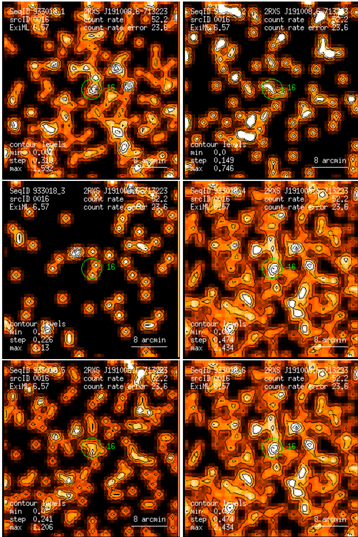
Figure 16: RASS 933018: detection 0016: band rate images, Gaussian filter: (1) PSPC channels 11 – 41, (2) 52 – 90, (3) 91 – 201, (4) 11 – 235, (5) 52 – 201, (6) 11 – 201. Broad band rates in counts/ks. Band rate contour levels in counts/ks/arcmin 2 .
