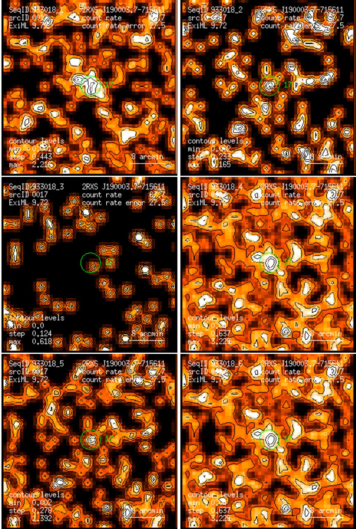
Figure 17: RASS 933018: detection 0017: band rate images, Gaussian filter: (1) PSPC channels 11 – 41, (2) 52 – 90, (3) 91 – 201, (4) 11 – 235, (5) 52 – 201, (6) 11 – 201. Broad band rates in counts/ks. Band rate contour levels in counts/ks/arcmin 2 .
