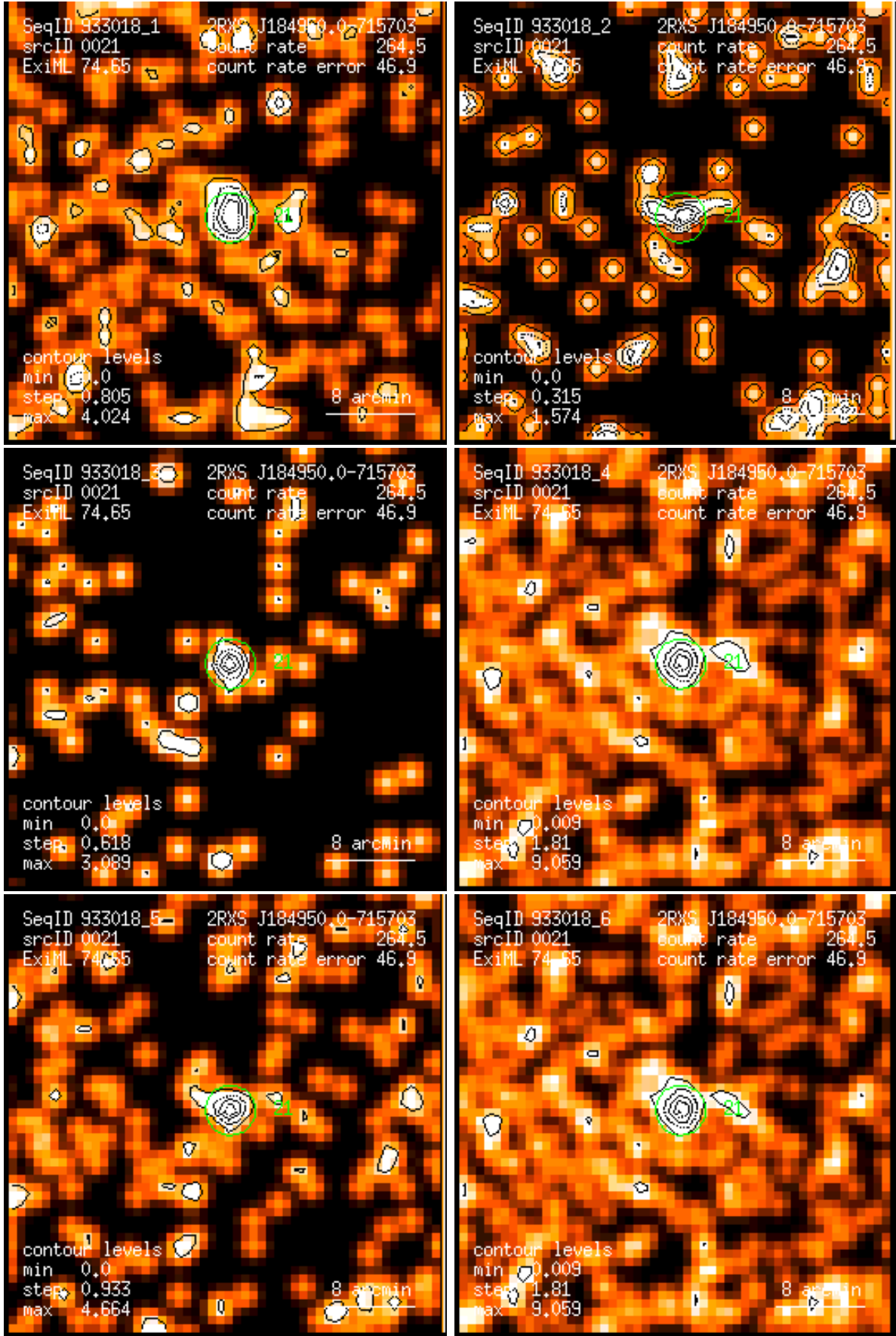
Figure 21: RASS 933018: detection 0021: band rate images, Gaussian filter: (1) PSPC channels 11 – 41, (2) 52 – 90, (3) 91 – 201, (4) 11 – 235, (5) 52 – 201, (6) 11 – 201. Broad band rates in counts/ks. Band rate contour levels in counts/ks/arcmin 2 .
