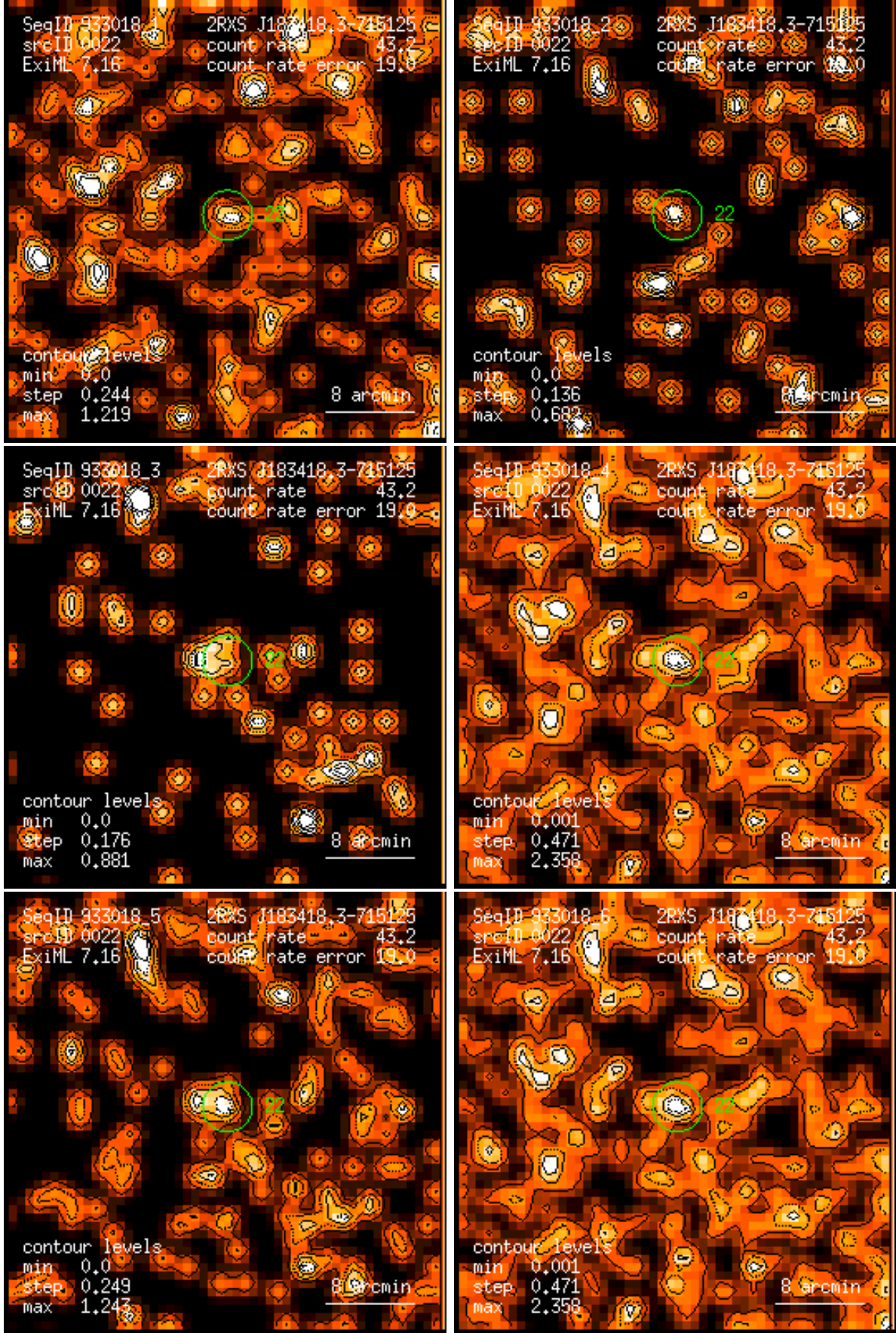
Figure 22: RASS 933018: detection 0022: band rate images, Gaussian filter: (1) PSPC channels 11 – 41, (2) 52 – 90, (3) 91 – 201, (4) 11 – 235, (5) 52 – 201, (6) 11 – 201. Broad band rates in counts/ks. Band rate contour levels in counts/ks/arcmin 2 .
