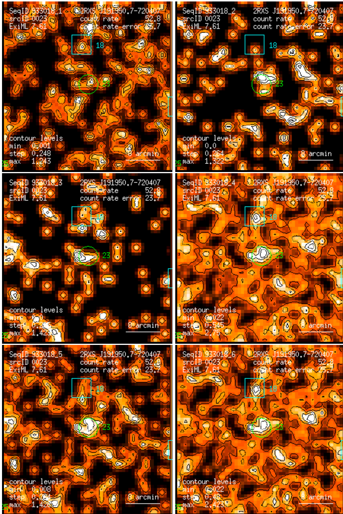
Figure 23: RASS 933018: detection 0023: band rate images, Gaussian filter: (1) PSPC channels 11 – 41, (2) 52 – 90, (3) 91 – 201, (4) 11 – 235, (5) 52 – 201, (6) 11 – 201. Broad band rates in counts/ks. Band rate contour levels in counts/ks/arcmin 2 .
