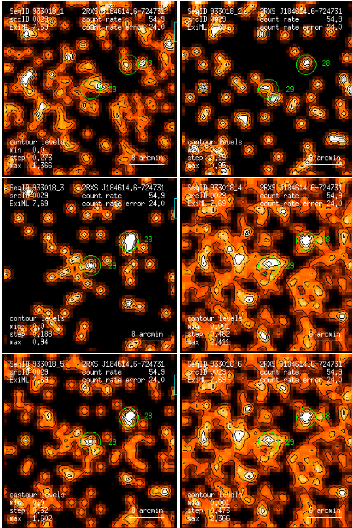
Figure 29: RASS 933018: detection 0029: band rate images, Gaussian filter: (1) PSPC channels 11 – 41, (2) 52 – 90, (3) 91 – 201, (4) 11 – 235, (5) 52 – 201, (6) 11 – 201. Broad band rates in counts/ks. Band rate contour levels in counts/ks/arcmin 2 .
